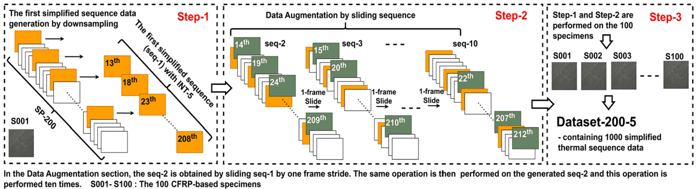
Fig. 3. The generation process of Dataset-200-5. On each specimen, the first simplified sequence data is created by a downsampling with the interval of 5 frames on the original thermal sequence span of SP-200. Then a sliding-sequence data augmentation operation is performed based on the first generated sequenced data, and 10 simplified sequences are obtained for each specimen. The abovementioned process is performed on the 100 specimens and a total of 1000 sequence data are gained to form this dataset.
