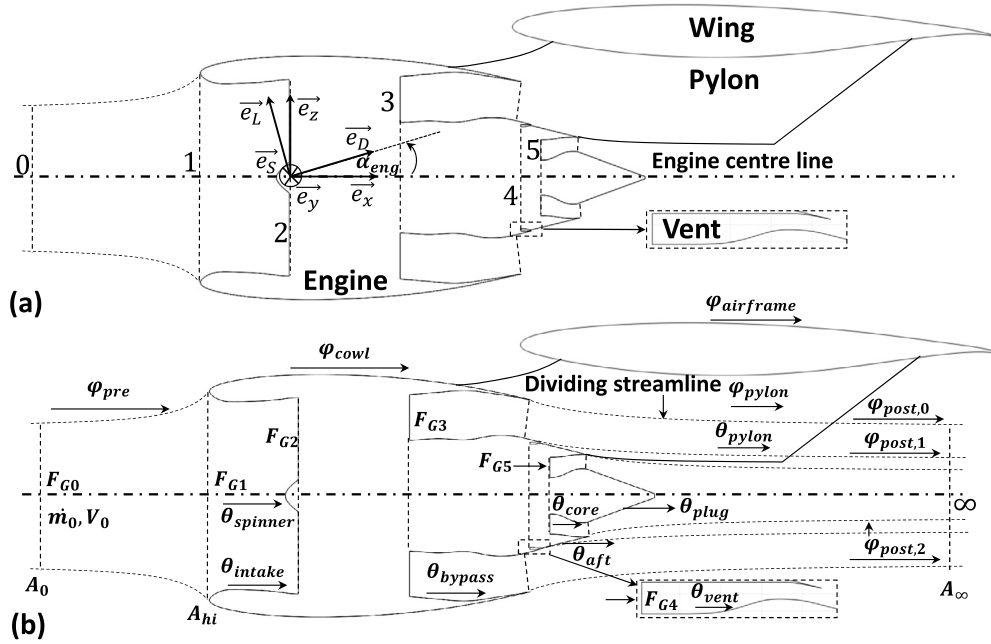
Fig. 3. Thrust and drag accounting system for installed turbofans with separate-jet exhausts: (a) Reference coordinate systems and engine station numbering, and (b) distribution of gauge stream, wall, and streamline aerodynamic forces.
