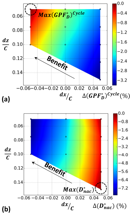
Fig. 10. Variation of normalised exhaust and nacelle performance: (a) modified gross propulsive force \Delta(GPF_D^*)^{Cycle}(\%) , and (b) modified nacelle drag \Delta(D_{nac}^*)^{Cycle}(\%) .
