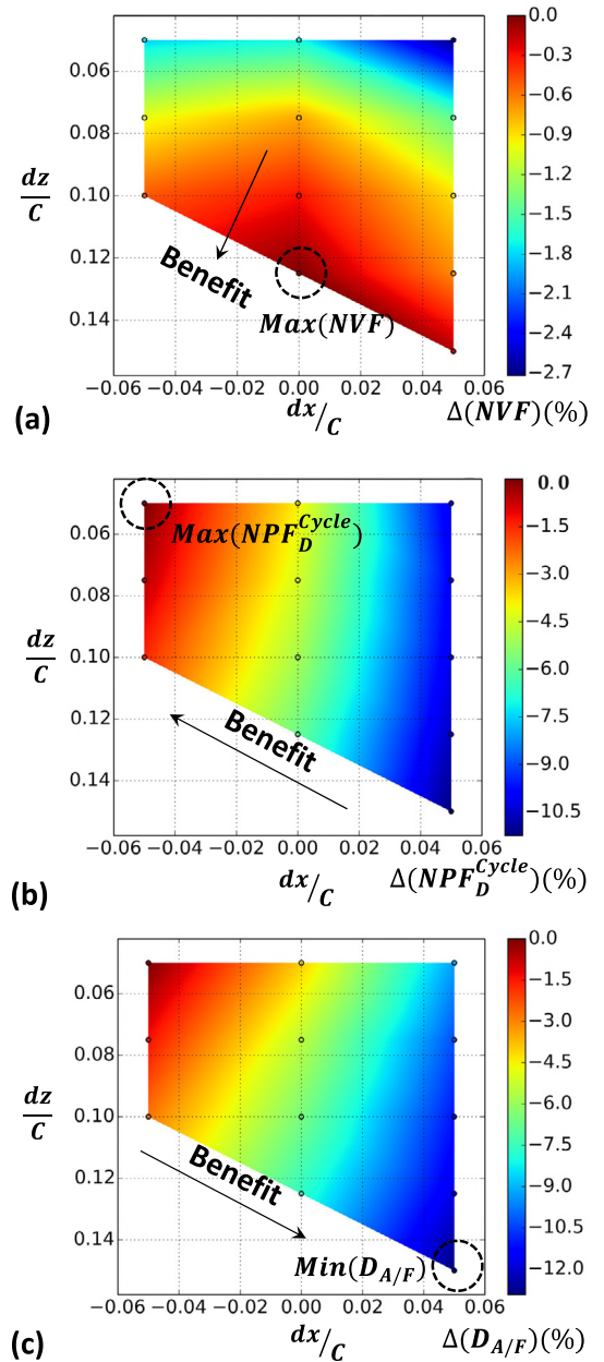
Fig. 9. Variation of coupled airframe-engine aerodynamic performance: (a) net vehicle force \Delta(NVF)(\%) , (b) net propulsive force \Delta(NPF_D^{Cycle})(\%) , and (c) airframe drag \Delta(D_{A/F})(\%) .
