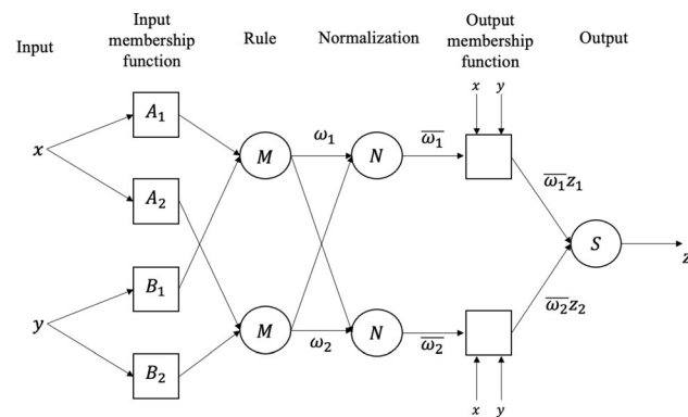
Fig. 9 ANFIS architecture [36]
