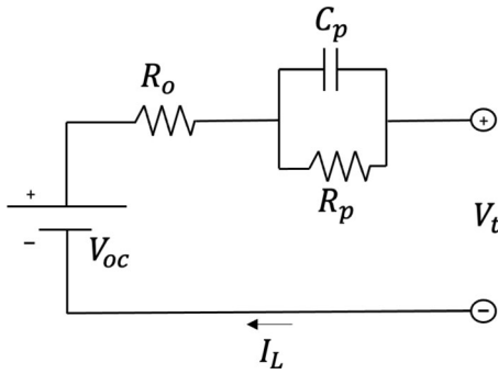
Fig. 5 First-order Thevenin RC network battery model
