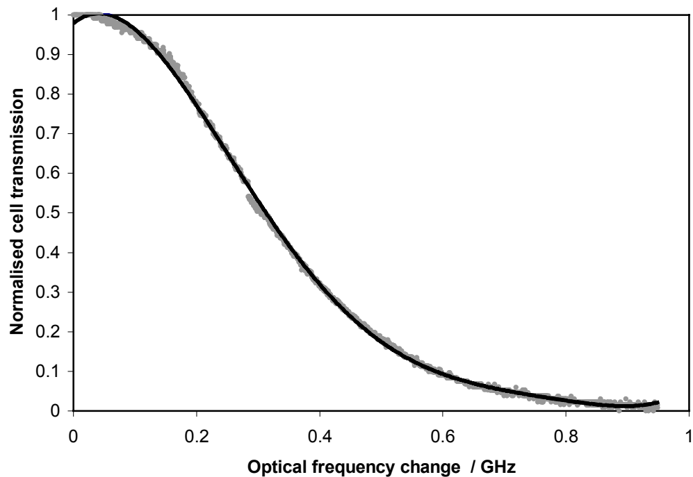
Figure 3: Plot showing the normalised transmission of the iodine vapour cell as a function of laser frequency (circles), and a sixth-order polynomial fit to the data (solid line).
