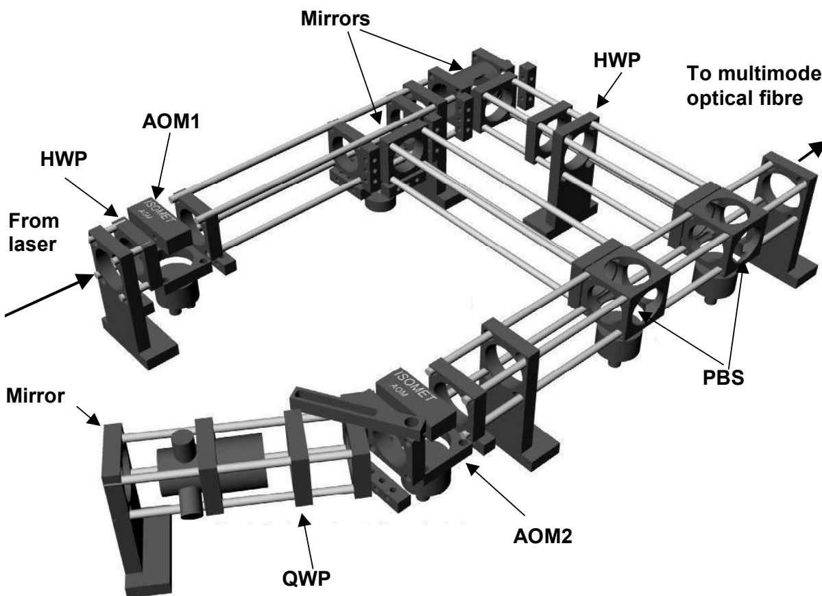
Figure 2: 3-D representation of the dual illumination configuration; HWP – half-wave plate, QWP – quarter-wave plate, AOM – acousto-optic modulator, PBS – polarising beam splitter.
