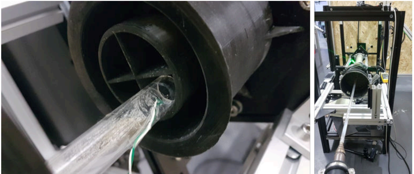
Figure 9. Glas tube inserted in one of the channels of the swirl generator for insertion of a hot flow streak. The cables sleeves visible are for a temperature sensor mounted at the tip of the glas tube(left). Inlet configuration for hot streak measurments with glas tube inserted in one of the channels of the swirler (right).
