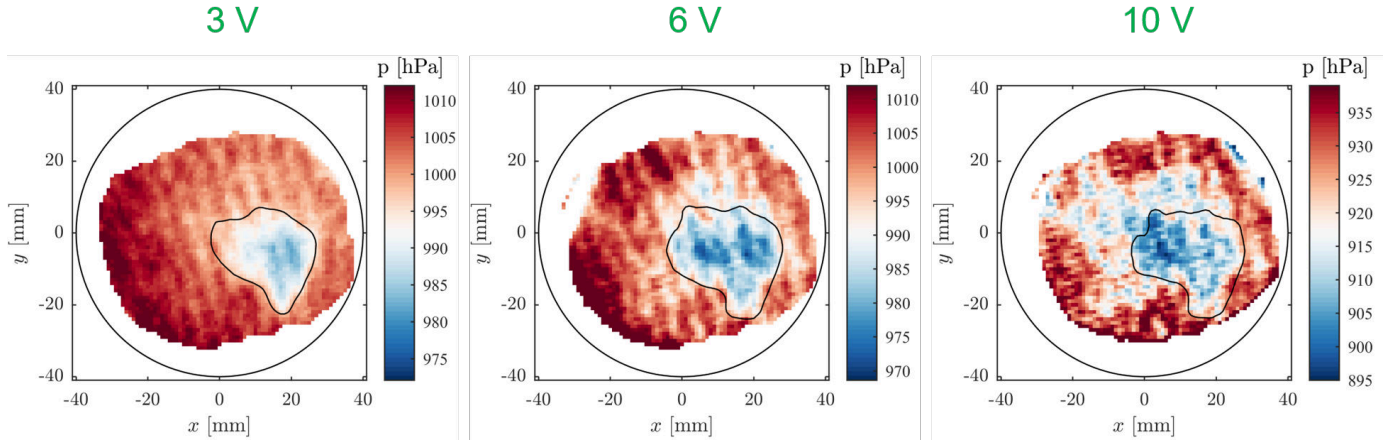
Figure 12. Pressure distribution measured by FRS behind a hot temperatur streak inserted in one of the swirl generators channels. Nominal velocity 30 m/s (left), 60 m/s (center) and 100 m/s (right).
