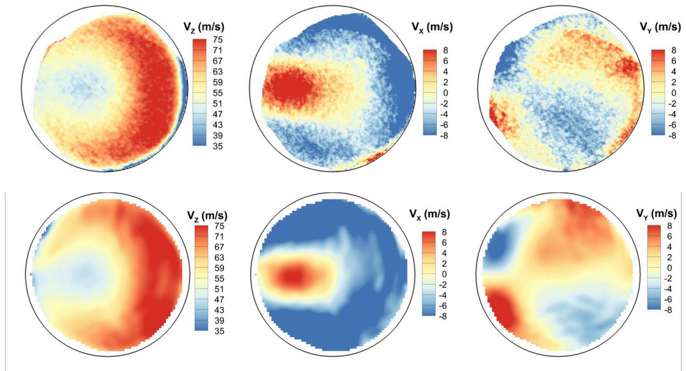
Figure 16. Time-averaged distribution maps of the 3D velocity field measured by FRS at the AIP of the CCITF for a Machnumber of 0.27 (top). Time-averaged distribution maps of the 3D velocity field measured by PIV (bottom). The averaging is done for 20'000 timesteps for PIV.
