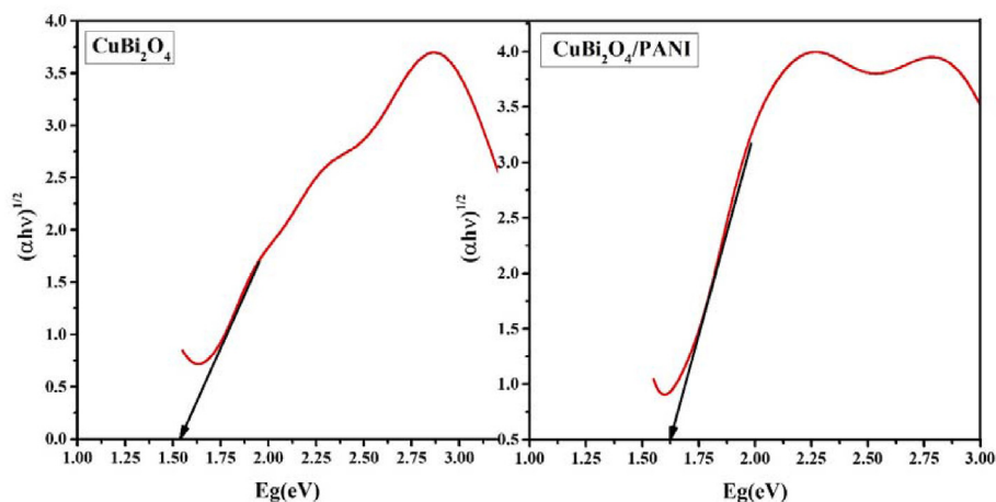
Figure 7. Tauc plot of \text{CuBi}_2\text{O}_4 and \text{CuBi}_2\text{O}_4/\text{PANI} composites.
