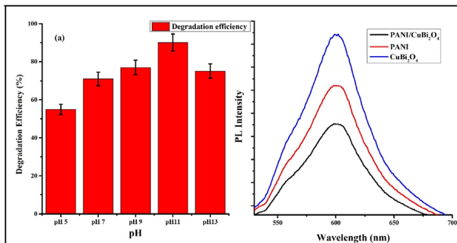
Figure 10. Effect of pH on the photodegradation of ammonia (a) and PL spectra of the photocatalyst to check the recombination behaviour of electron and holes (b).
