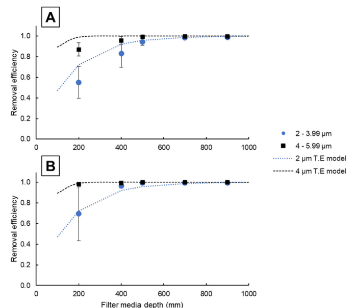
Fig. 6. Filter removal efficiency following surface agitation at various media depths after: (A) one bed volume of flow, and (B) six bed volumes of flow, for particle size ranges 2–3.99 \mu\text{m} and 4–5.99 \mu\text{m} . The T.E. model is the model developed by Tufenkji and Elimelech (2004).
