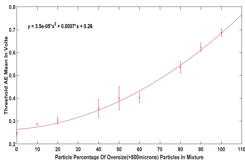
Figure 7. Correlation plot of oversize particles against AE amplitude mean with R = 0.97 .
