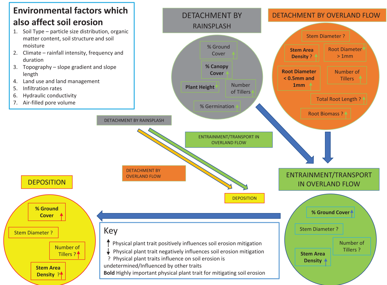
FIGURE 1 Soil erosion processes as affected by plant traits
