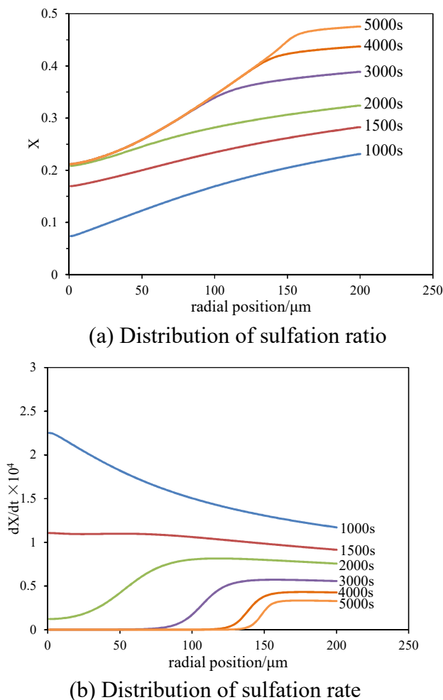
Fig. 8 Distribution of sulfation ratio and sulfation rate
