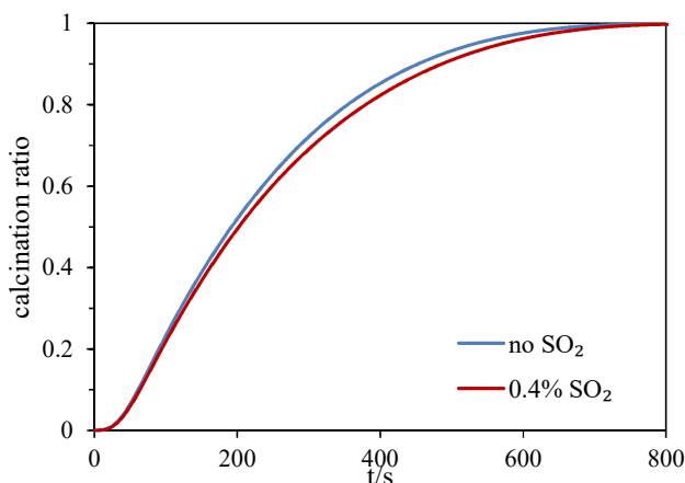
Fig. 5 Effect of \text{SO}_2 on calcination of limestone
