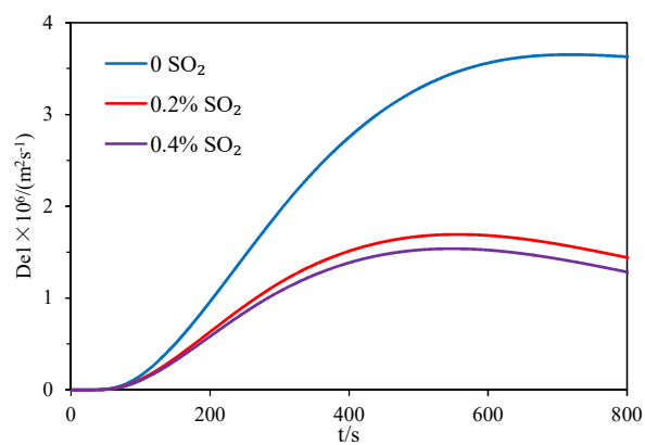
Fig. 7 Effect of \text{SO}_2 on the effective diffusion coefficient of \text{CO}_2 in pore
