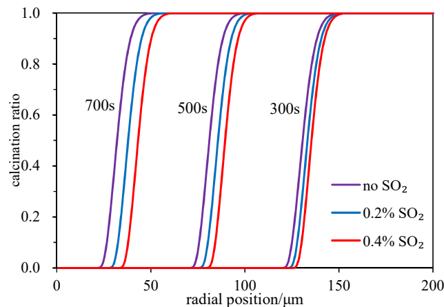
Fig. 6 Effect of \text{SO}_2 on the distribution of calcination ratio
