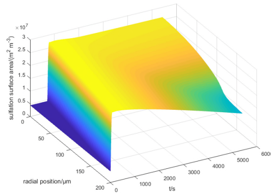
Fig. 9 Surface area for the sulfation reaction
