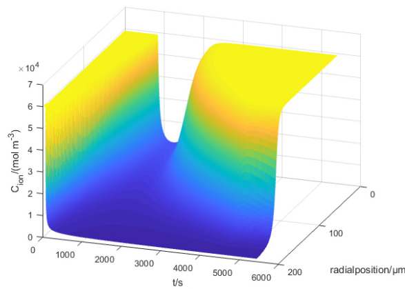
Fig. 10 \text{Ca}^{2+} ion concentration on the sulfation surface
