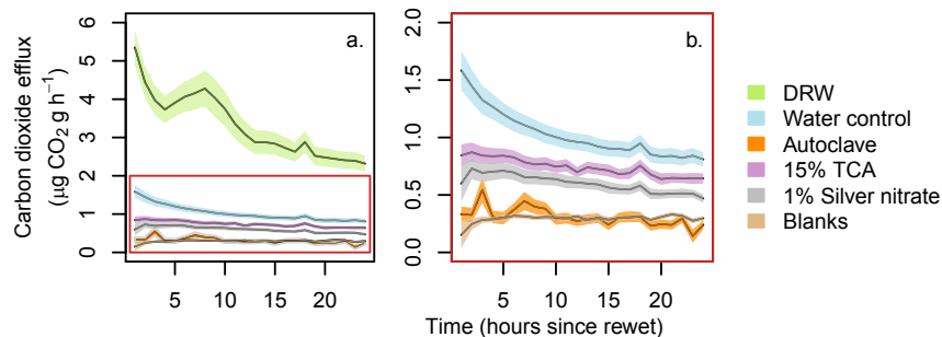
Fig. 3. CO 2 efflux rates following rewetting of a dry soil with various solutions; (a) live soil (green) exposed to a DRW cycle compared to all other treatments including a moist control (blue), area outlined in red is shown in greater detail in (b); (b) amplification of y-axis from (a), i.e. CO 2 efflux following a DRW cycle from the moist control (blue), blanks (no soil - brown), autoclaved (orange), 15% TCA (purple) and 1% silver nitrate (grey) treated soils. Lines show mean rates of CO 2 efflux (n = 12 (3 reps each of 4 soils)) surrounded by confidence bands of \pm 1 standard error.
