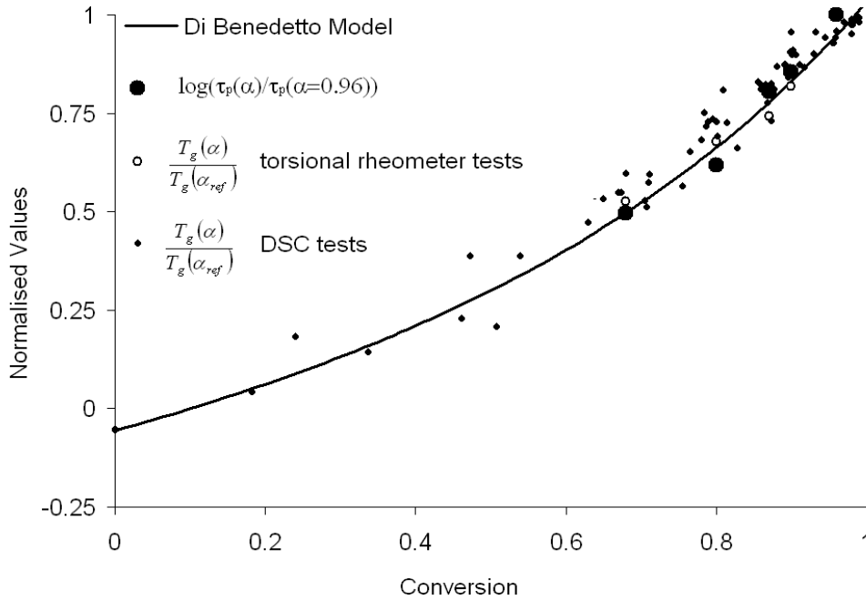
Figure 6 - Normalized values of single relaxation time vs conversion with normalized values of glass transition temperature obtained experimentally by thermal analysis and torsional rheometry alongside the Di Benedetto model (solid line)
