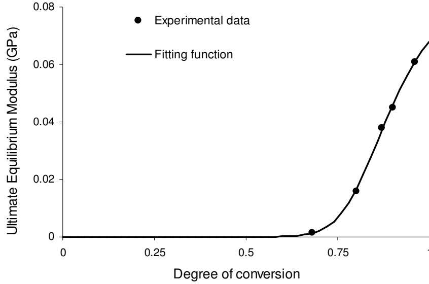
Figure 1 - Experimental points and fitting curve for ultimate relaxed modulus
