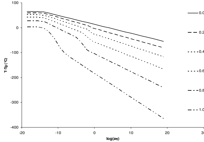
Figure 4 – (a) Experimental shift factor data vs. (T - T_g) and model fitting at each conversion (b) Model predictions over the full degree of cure range
