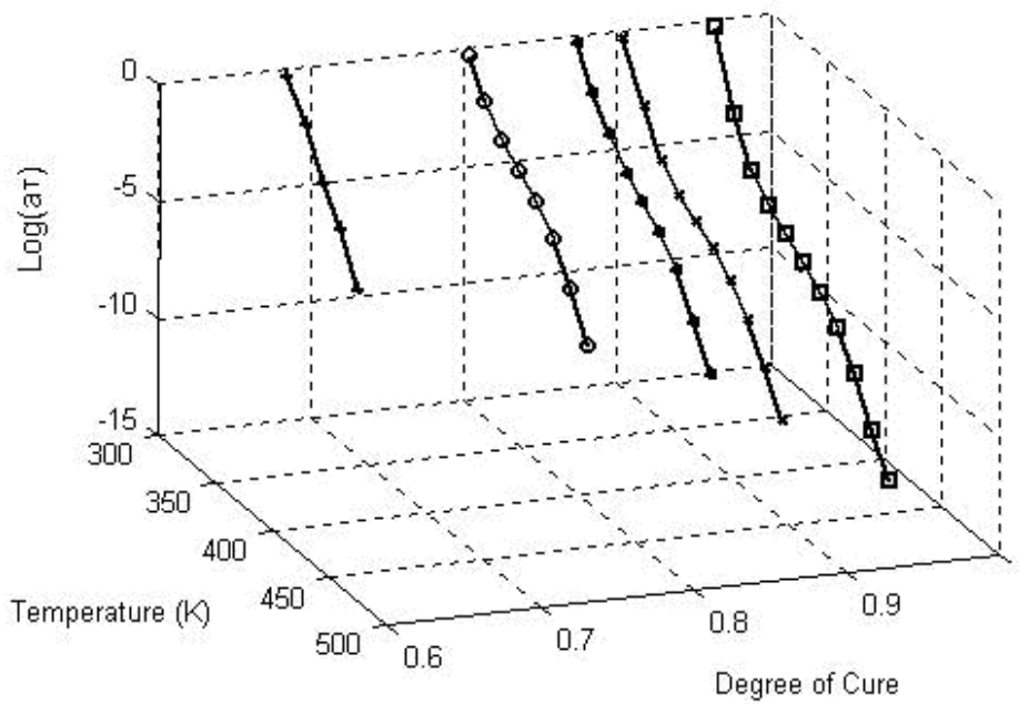
Figure 2 - 3D plot of experimental shift factors vs. temperature and degree of cure
