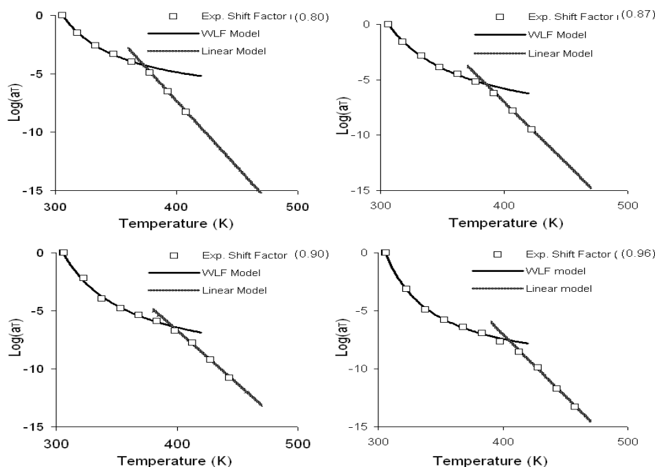
Figure 3 - Shift factors for partially cured samples (0.80- 0.87-0.90-0.96) fitted with WLF and linear models
