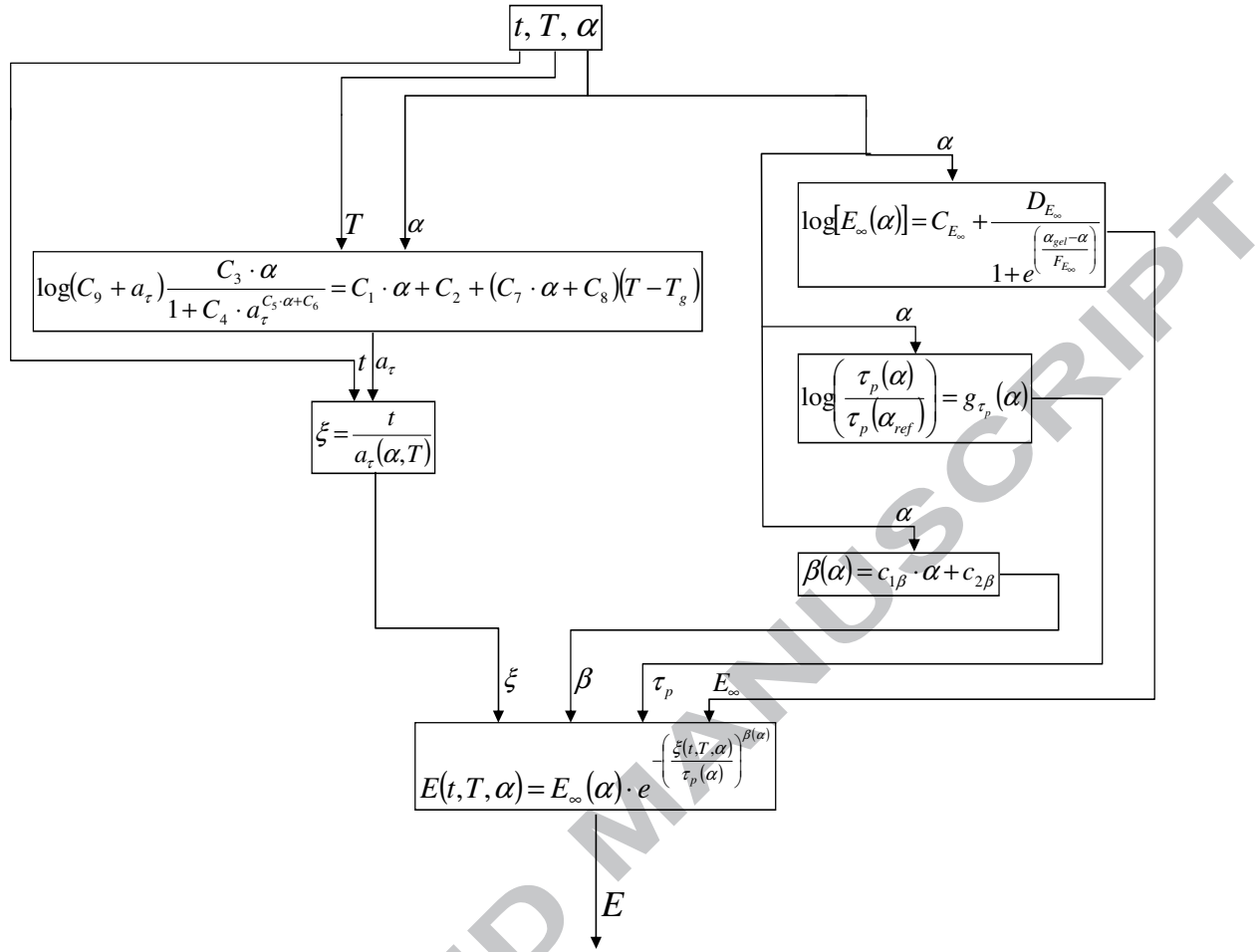
Figure 8 – Sub-model schematic.
