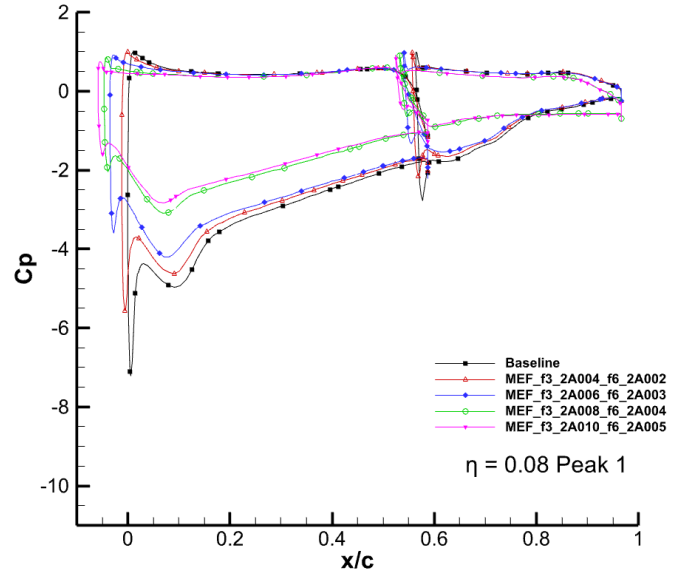
Fig. 11 Comparison of the pressure distributions of amplitude configurations at h/c=0.224
