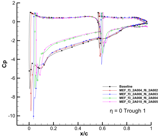
Fig. 11 Comparison of the pressure distributions of amplitude configurations at h/c=0.224
