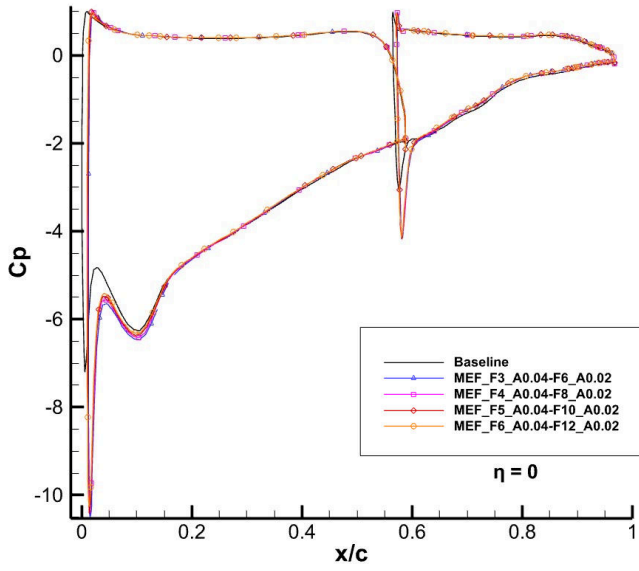
Fig. 12 Pressure distribution plots of the frequency configurations at h/c=0.134
