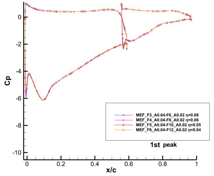
Fig. 12 Pressure distribution plots of the frequency configurations at h/c=0.134
