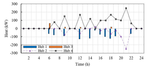
Fig. 12. Heat P2P trading under case 3.
