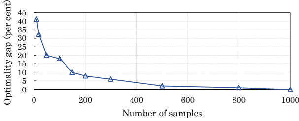
Fig. 18. Convergence characteristics of the proposed BOTH model.
