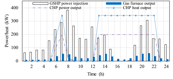
Fig. 15. Converter scheduling result of case 2.
