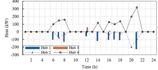
Fig. 10. Heat P2P trading under case 1.
