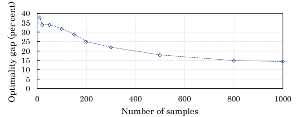
Fig. 17. Convergence characteristics of the MDRTH model.
