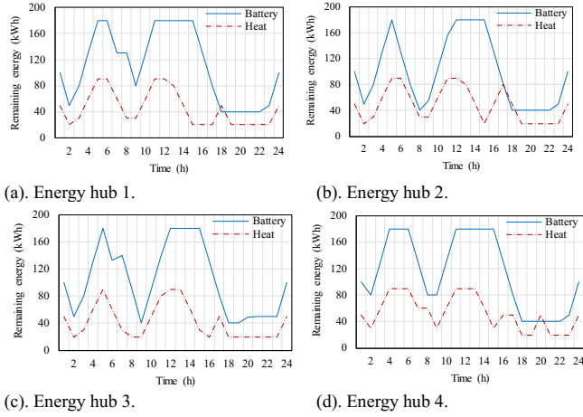
Fig. 13. Remaining capacity of battery and heat storage.
