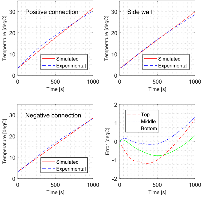
Figure 11: Temperature profile at 0°C ambient temperature.
