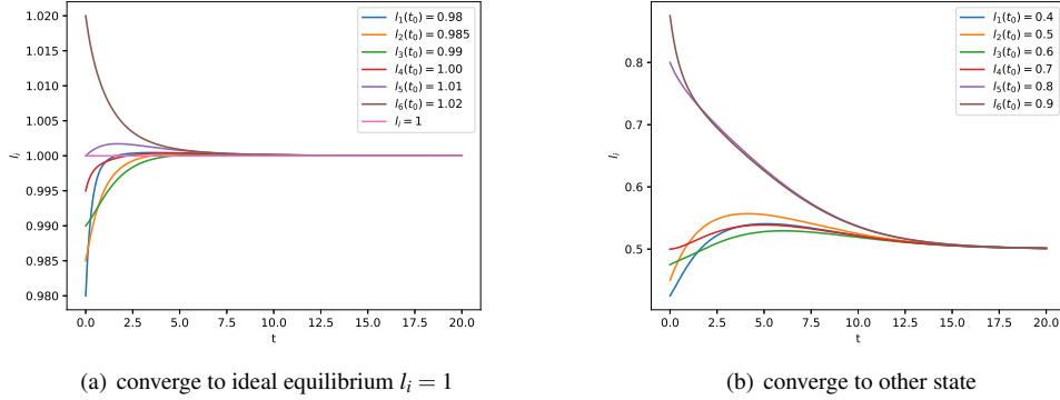
FIG. 7. These two figures show the dynamics process of each node with different initial values. In (a), the initial value of each node belongs to the ROA, then each node converges to the ideal equilibrium l_i = 1 at last. While, in (b), the initial values of nodes do not belong to the ROA, then these nodes converge to another state at last.
