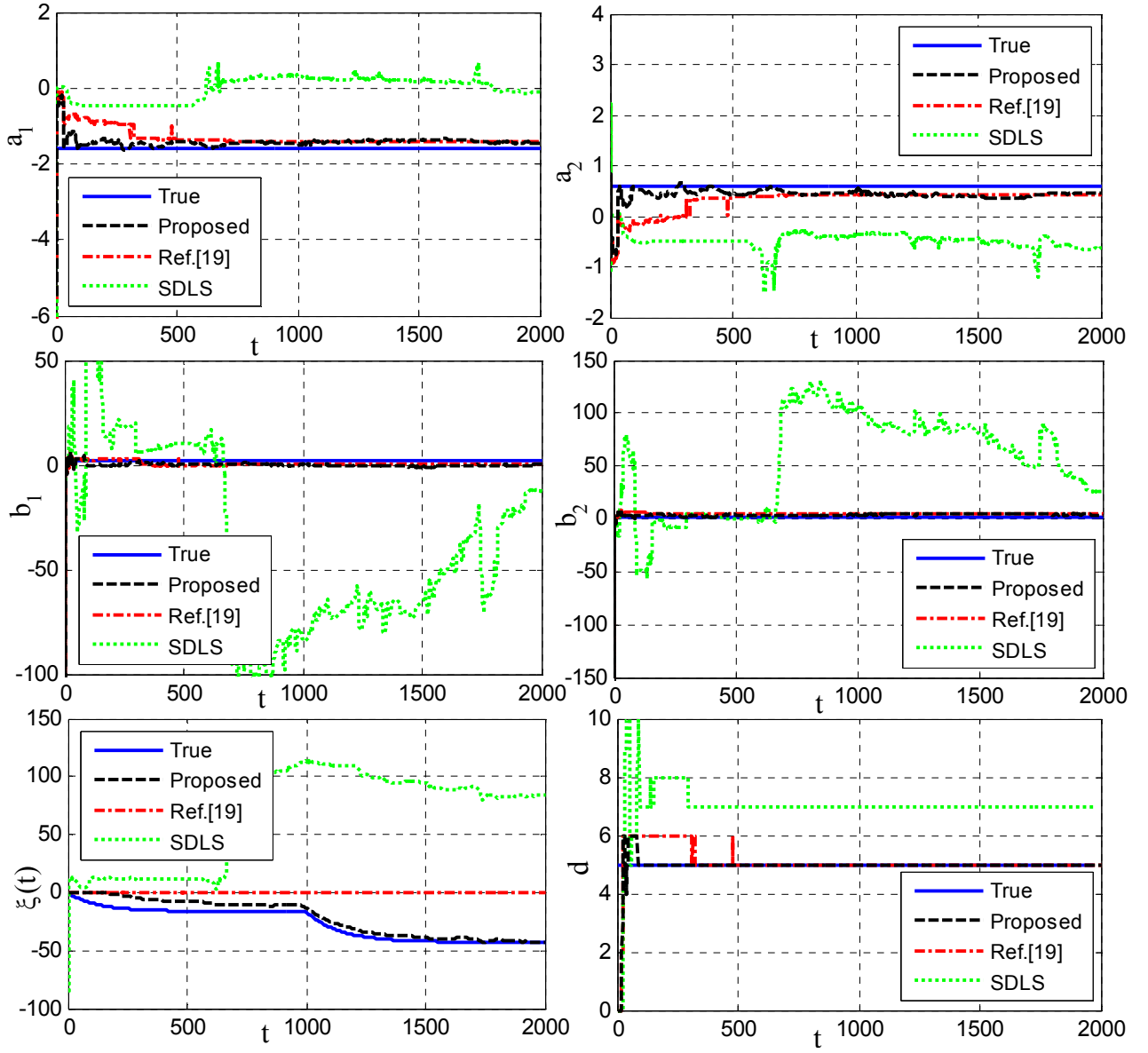
Fig. 8. Identification results using different algorithms for Example 3
