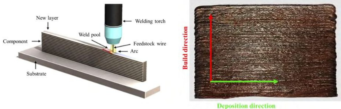
a) Schematic of WAAM (reprinting permission for these images has been obtained from the publishers [38]).
