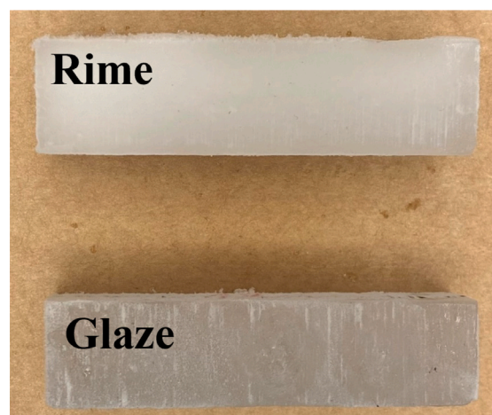
Fig. 1. Photograph of typical Rime ice and Glaze ice specimens; 60 mm in length and 15 mm by 15 mm in cross-section.
