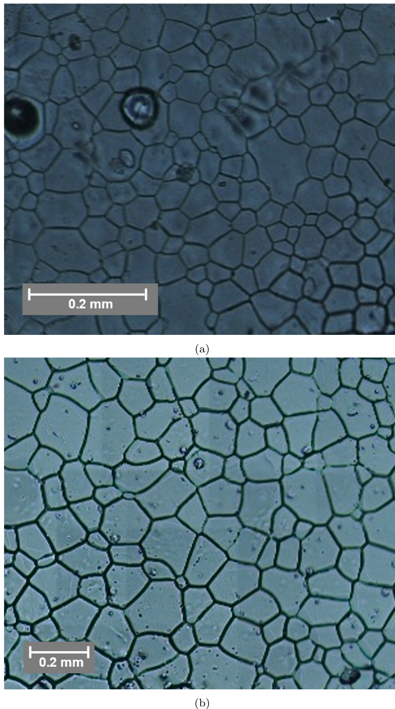
Fig. 2. Optical micrographs of (a) Rime ice and (b) Glaze ice, taken at the interface using a replicate technique [22].
