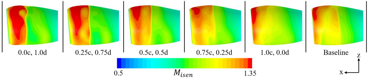
Figure 6: Isentropic Mach number contour plots for the optimised and baseline designs at the cruise condition. Shown for the 45DoF configuration only. All multi-point weightings shown (c - Cruise, d - Diversion)
