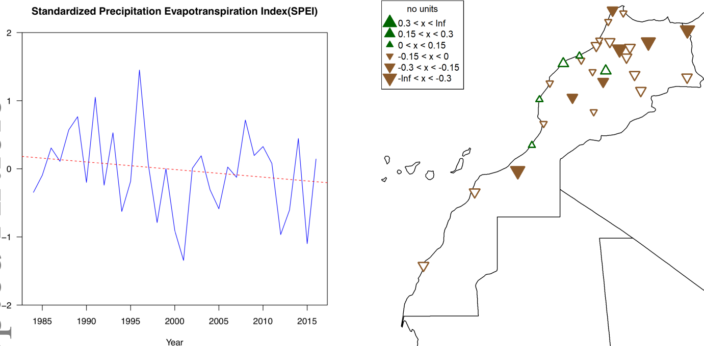
Figure 4: Trends in the SPEI at the country scale (left panel) and at individual stations (per decade) across Morocco (right map). The green and brown colours indicate positive and negative trends respectively. Statistically significant trends at 5% confidence interval are represented by solid triangles. The size of the triangles is proportional to the magnitude of the trend.
