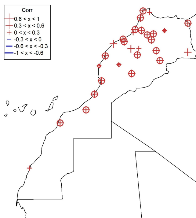
Figure 5: Correlations between NAO index and climate indices at station level and for winter Dec-Feb (NCMP2, WNights, CNights and SPEI), Oct-Feb (NCMP2) and annually (NCMP2). Circles indicate significant correlations at 5% level. Correlations at station level are calculated over the available period of each station (see Table 1).
