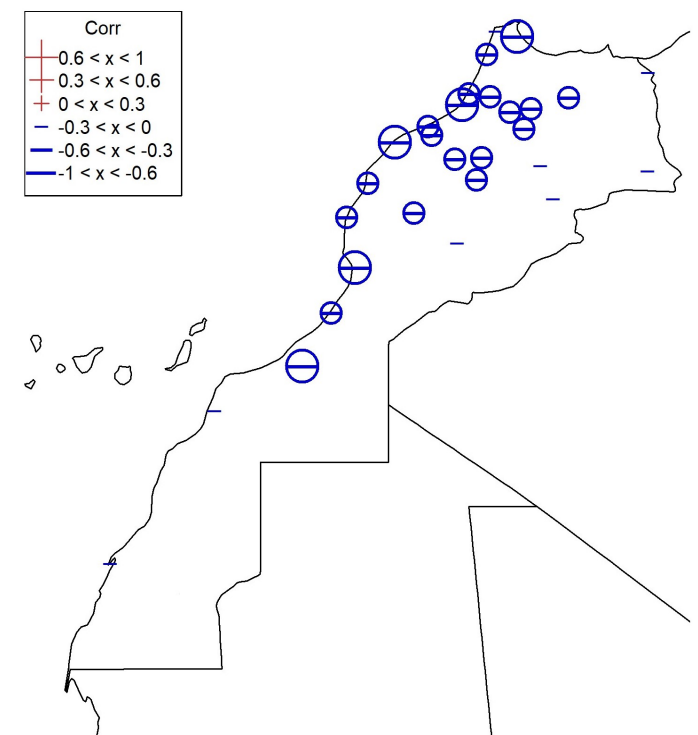
Figure 5: Correlations between NAO index and climate indices at station level and for winter Dec-Feb (NCMP2, WNights, CNights and SPEI), Oct-Feb (NCMP2) and annually (NCMP2). Circles indicate significant correlations at 5% level. Correlations at station level are calculated over the available period of each station (see Table 1).
