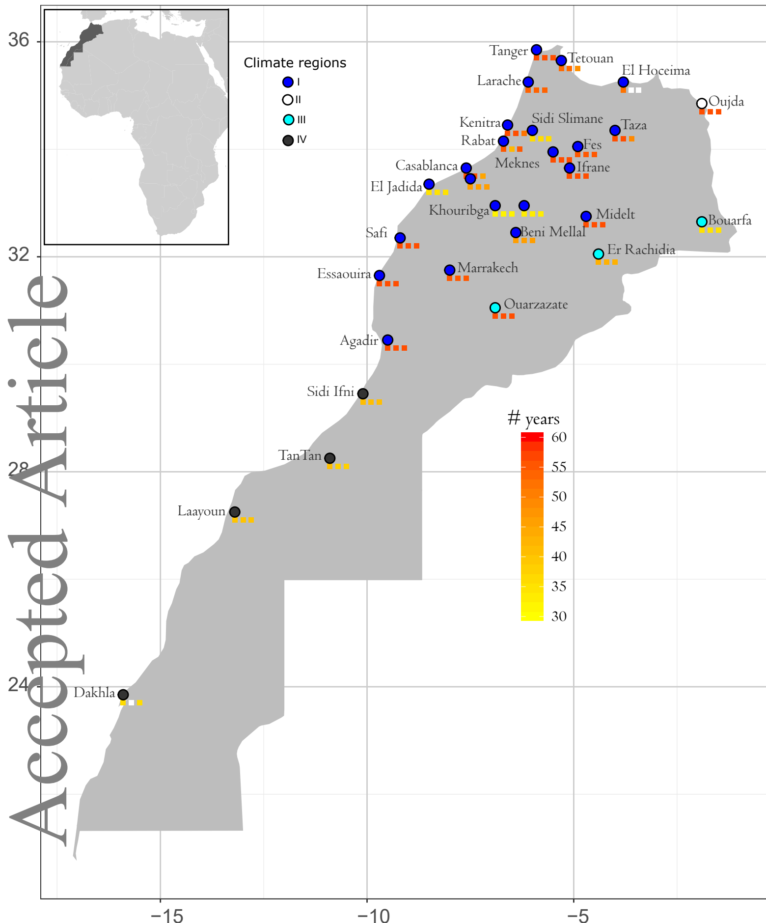
Figure 1: Geographical distribution of stations used in this study and their record lengths. Circles indicate the location and the name of the station with fill colours showing climate regions they belong to. The colours of the squares at each station indicate the record length (after homogeneity tests) of the precipitation, maximum and minimum temperature time series respectively from left to right. White boxes indicate the series that are truncated after homogeneity check and have less than 30 years (i.e. Dakhla truncated in at 2004 and Tmax and T min are not considered for AlHoceima station)
