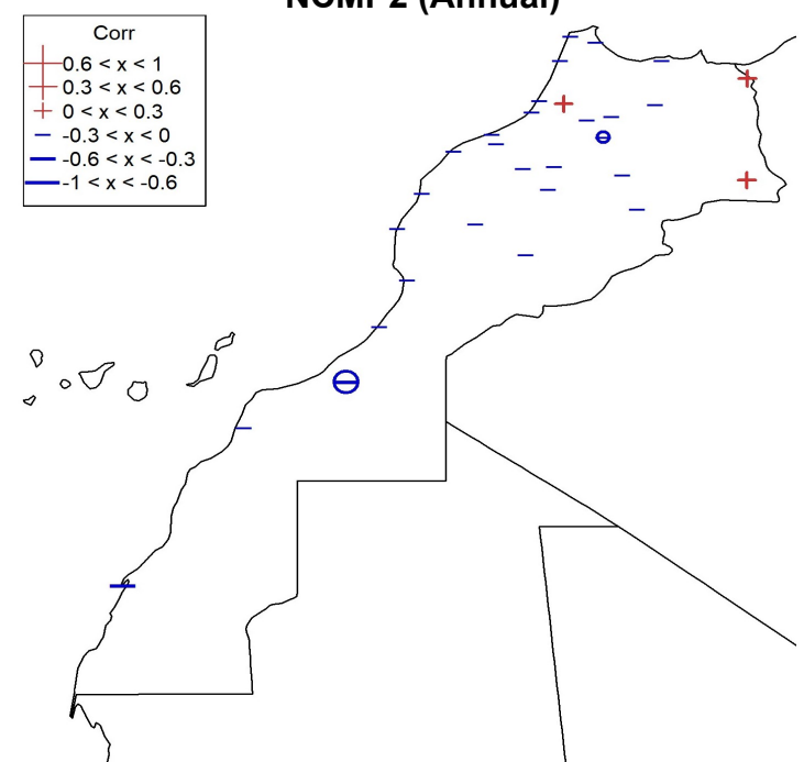
NCMP2 (Annual)
