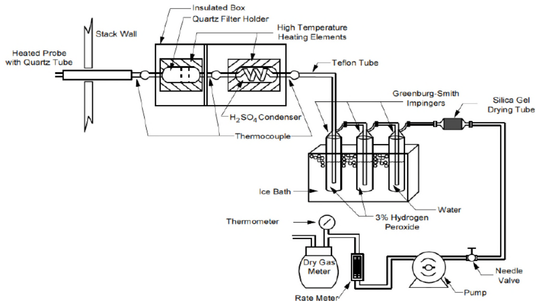
Figure 5 The modified controlled condensation method (CCM) \text{SO}_3 sampling scheme. 106
