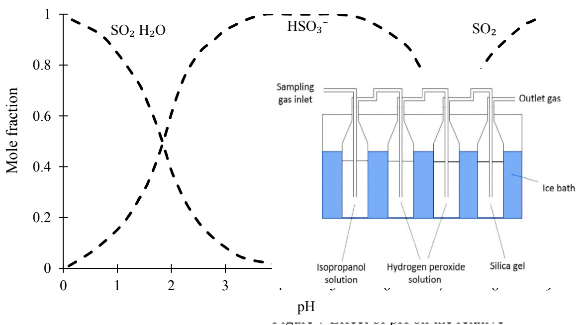
Figure 6 Effect of pH on the relative concentrations of the SO 2 species in solution 108
