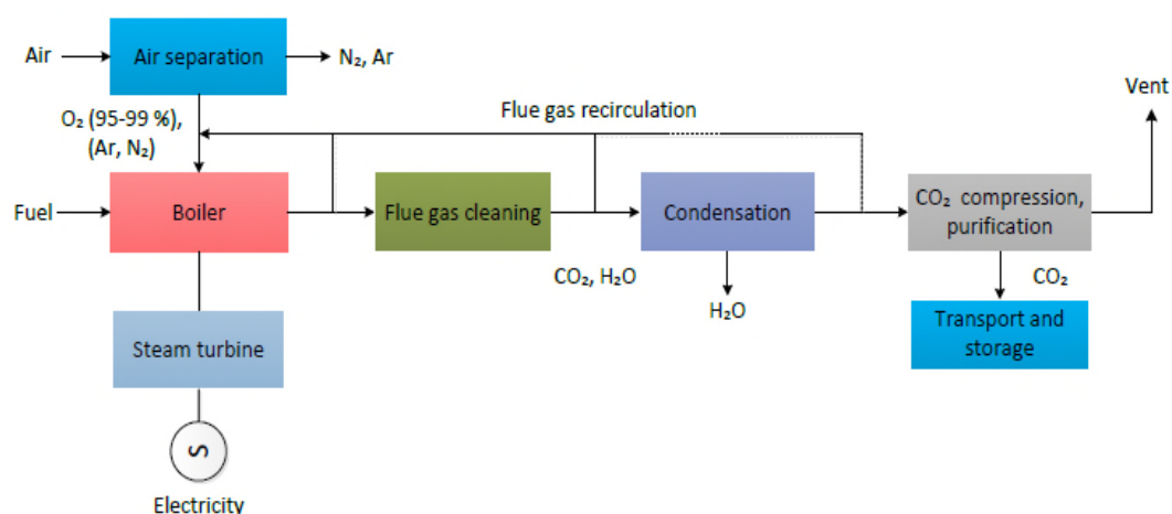
Figure 1 Principal scheme of oxy-fuel combustion process
