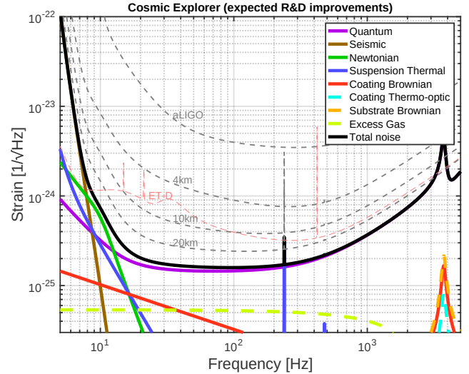
FIG. 1. Target sensitivity for a next generation gravitational-wave detector, known as “Cosmic Explorer” for its ability to receive signals from cosmological distances. The solid curves are for a 40 km long detector, while the dashed grey curves show the sensitivity of shorter, but technologically similar detectors; lengths are 4, 10 and 20 km. The Advanced LIGO and Einstein Telescope design sensitivities are also shown for reference.
