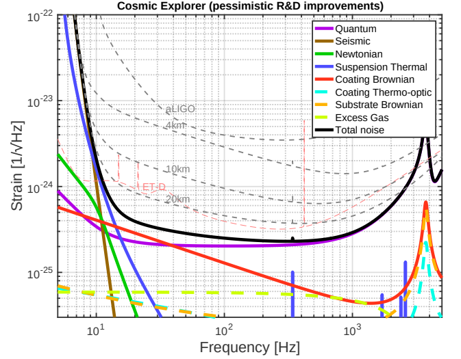
FIG. 3. Similar to figure 2 but with coating and suspension thermal noise models which assume minimal progress. The wide-band signal extraction choice is made to minimize the impact of CTN. The proximity of the dashed grey 4 km curve to the Advanced LIGO reference curve reflects the fact that coating technology, which is nearly limiting in Advanced LIGO, becomes dominant over a range of frequencies given the reduction of quantum noise assumed for the future.
