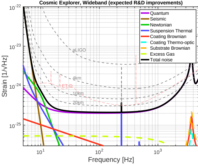
FIG. 2. Similar to figure 1 but with a more reflective signal extraction mirror which gives a wider sensitive band, but is less sensitive in-band. The tradeoff between in-band sensitivity and bandwidth will need to be optimized to maximize specific science objectives (e.g., testing general relativity with black hole binaries, measuring neutron star equation of state, detection of GW from supernovae, etc.). The dashed grey curves show the sensitivity of shorter, but technologically similar detectors; lengths are 4, 10 and 20 km.
