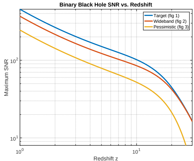
FIG. 4. The maximum signal-to-noise ratio (SNR) for which GW detectors with the sensitivities shown in figures 1, 2 and 3 would detect a system made of two black holes (each with an intrinsic mass 30 M_{\odot} ), as a function of redshift. Many systems of this sort will be detected at z < 2 with an SNR > 100 , enabling precision tests of gravity under the most extreme conditions.
