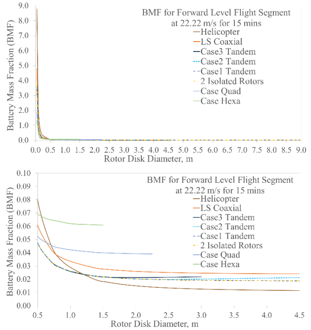
Fig. 14. Forward Levelled Flight (at 22.22 m/s for 15 mins) BMF vs Rotor Disk Diameter - 500 kg Titanian rotorcrafts. Top - BMF for rotor diameters from 0.05 to 9 m. Bottom - Close-up view, focusing on BMF for rotor diameters from 0.5 m to 4.5 m on the x-axis for clarity
