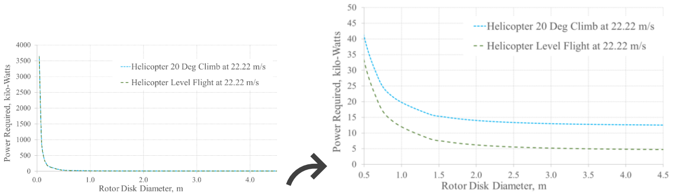
Fig. 10. Forward Flight Power Required (at 22.22 m/s) vs Rotor Disk Diameter - 500 kg Titanian Conventional Helicopter. Graph on the right side is the zoomed in view of the graph on left side, with rotor disk starting from 0.5 m.
