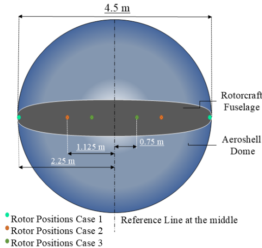
Fig. 2. Diagram of the positioning of rotor hubs of tandem rotorcraft Cases 1, 2, and 3, on the fuselage placed inside an aeroshell. (Not to scale)
