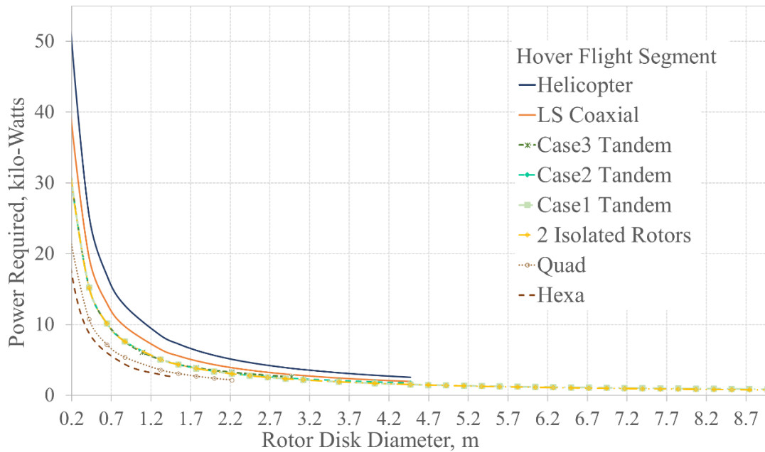
Fig. 8. Hover Power Required vs Rotor Disk Diameter (0.2 m to 9 m)– Comparison between various 500 kg rotorcraft configurations (Helicopter, Coaxial, Tandem Cases, 2 Isolated Rotors, Quadcopter)
