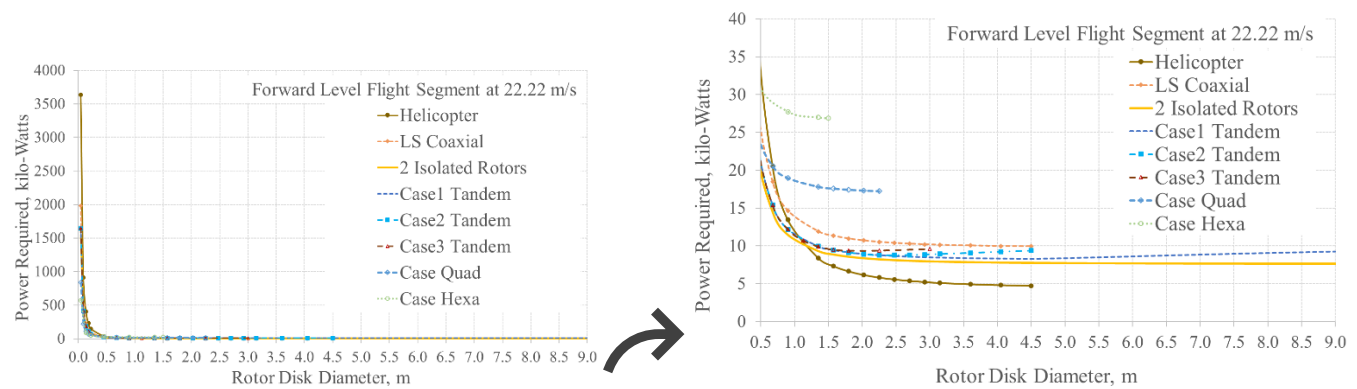
Fig. 11. Forward Level Flight Power Required (at 22.22 m/s) vs Rotor Disk Diameter - 500 kg Titanian Various Rotorcraft Configurations. Right-side graph is the zoomed in view of the left-side graph with rotor disk starting from 0.5 m.
