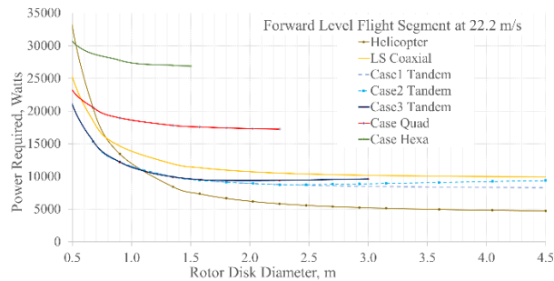
Fig. 16. Power Required (Forward Level at 22.22 m/s) vs Rotor Disk Diameter (Rotor Diameter Limits – 0.5 m to 4.5m) – Comparison between various 500 kg rotorcraft configurations
