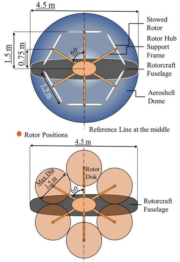
Fig. 5 Schematic illustration (not to scale) of the rotor hub positioning of hexarotor configuration with nonoverlapping equal-sized rotors. Top - stowed inside aeroshell. Bottom - operational mode
