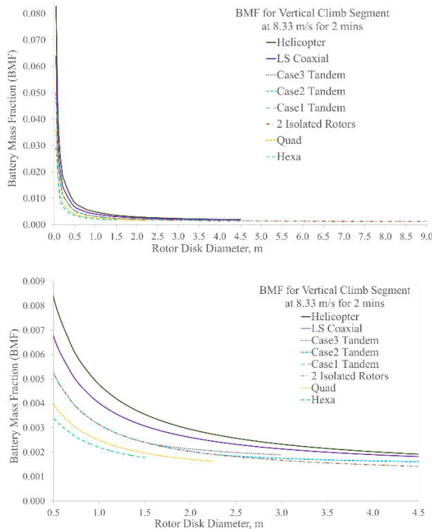
Fig. 13. Vertical Climb (at 8.33 m/s for 2 mins) BMF vs Rotor Disk Diameter - 500 kg Titanian rotorcrafts. Top - BMF for rotor sizes from 0.05 to 9 m. Bottom - Close-up view, focusing on BMF for rotor diameters from 0.5 m to 4.5 m on the x-axis for clarity
