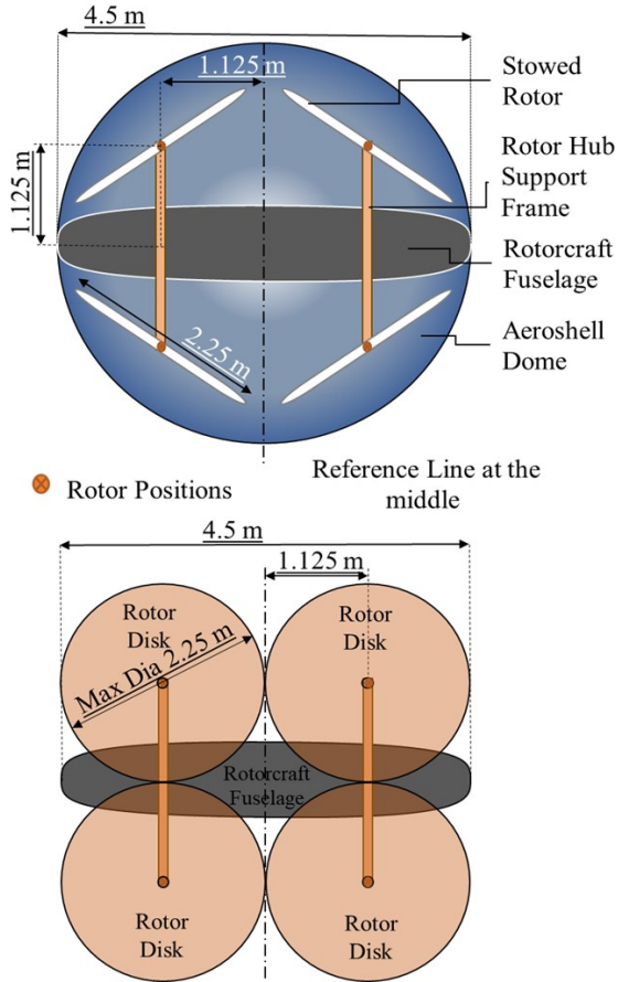
Fig. 4. Schematic illustration (not to scale) of the rotor hub positioning of Quadrotor configuration with nonoverlapping equal-sized rotors. Top - stowed inside aeroshell. Bottom - operational mode
