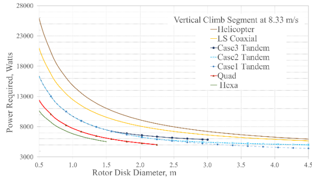
Fig. 15. Power Required (Vertical Climb at 8.33 m/s) vs Rotor Disk Diameter (Rotor Diameter Limits – 0.5 m to 4.5m) – Comparison between various 500 kg rotorcraft configurations
