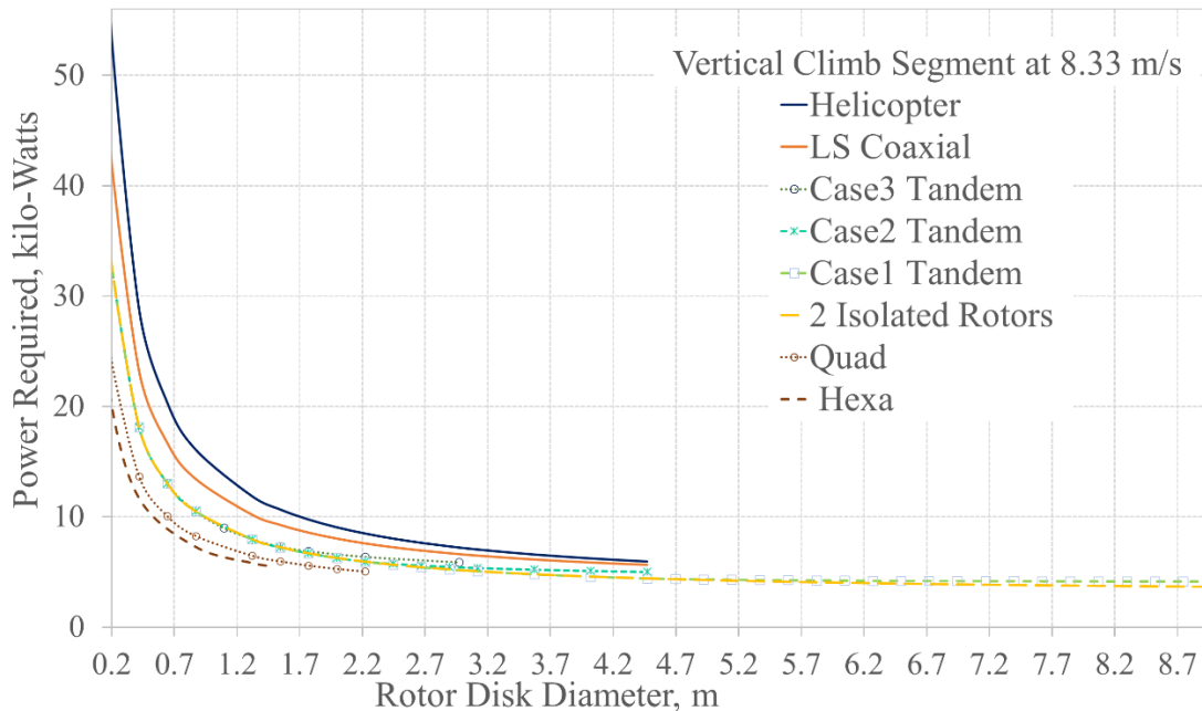
Fig. 9. Vertical Climb Power Required (at 8.33 m/s) vs Rotor Disk Diameter (0.2 m to 9 m)– Comparison between various 500 kg rotorcraft configurations (Helicopter, Coaxial, Tandem Cases, 2 Isolated Rotors, Quadcopter)
