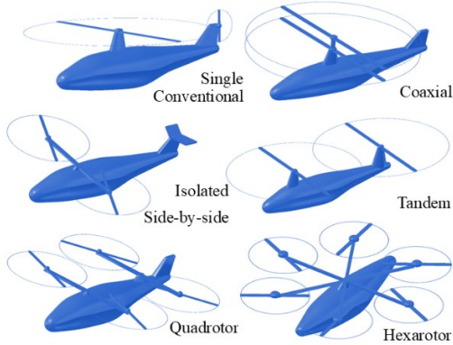
Fig. 1. Rotorcraft Configurations Illustration
