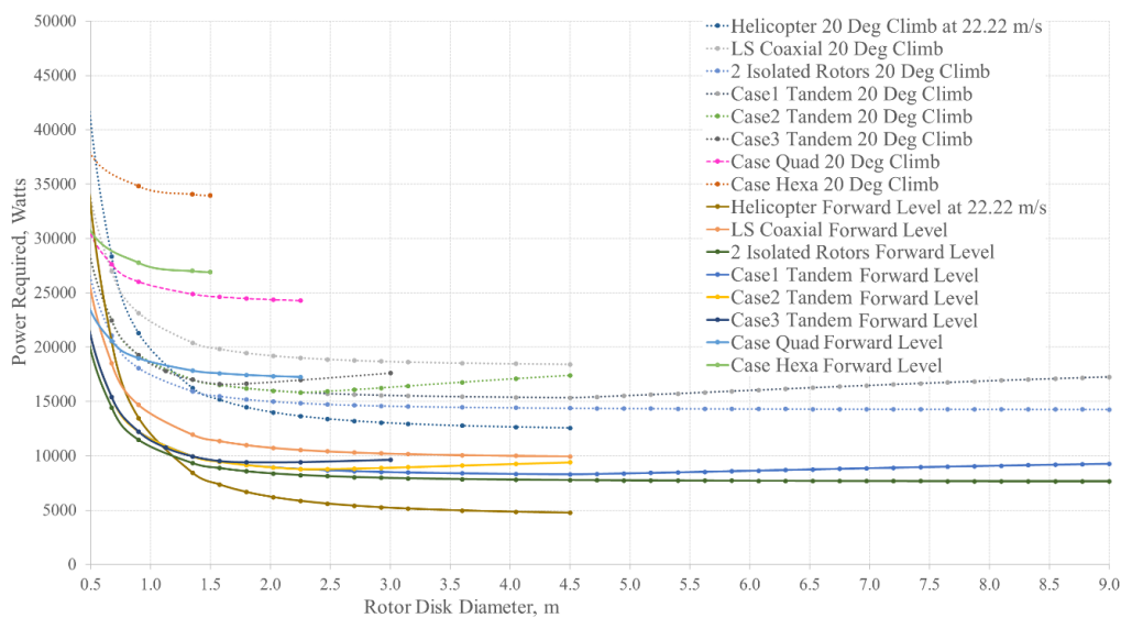
Fig. 12. Forward Flight Power Required (at 22.22 m/s) vs Rotor Disk Diameter (Rotor Diameter Limits – 0.5 m to 9 m) – Comparison between various 500 kg rotorcraft configurations (Helicopter, Coaxial, Tandem Cases, 2 Isolated Rotors, Quadcopter, Hexacopter)
