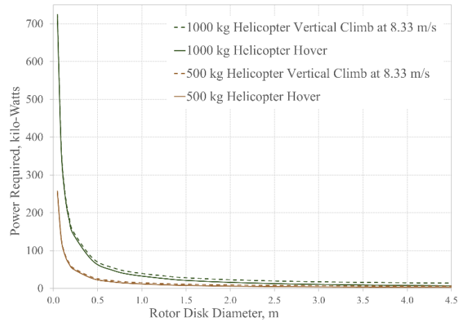
Fig. 7. Power Required vs Rotor Disk Diameter - 500 kg & 1000 kg Titanian Conventional Helicopter
