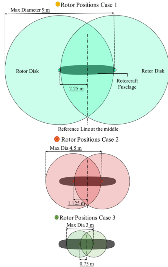
Fig. 3. Schematic illustration of the rotor positioning of tandem rotorcraft Cases 1, 2, and 3 in operational mode. (Not to scale)
