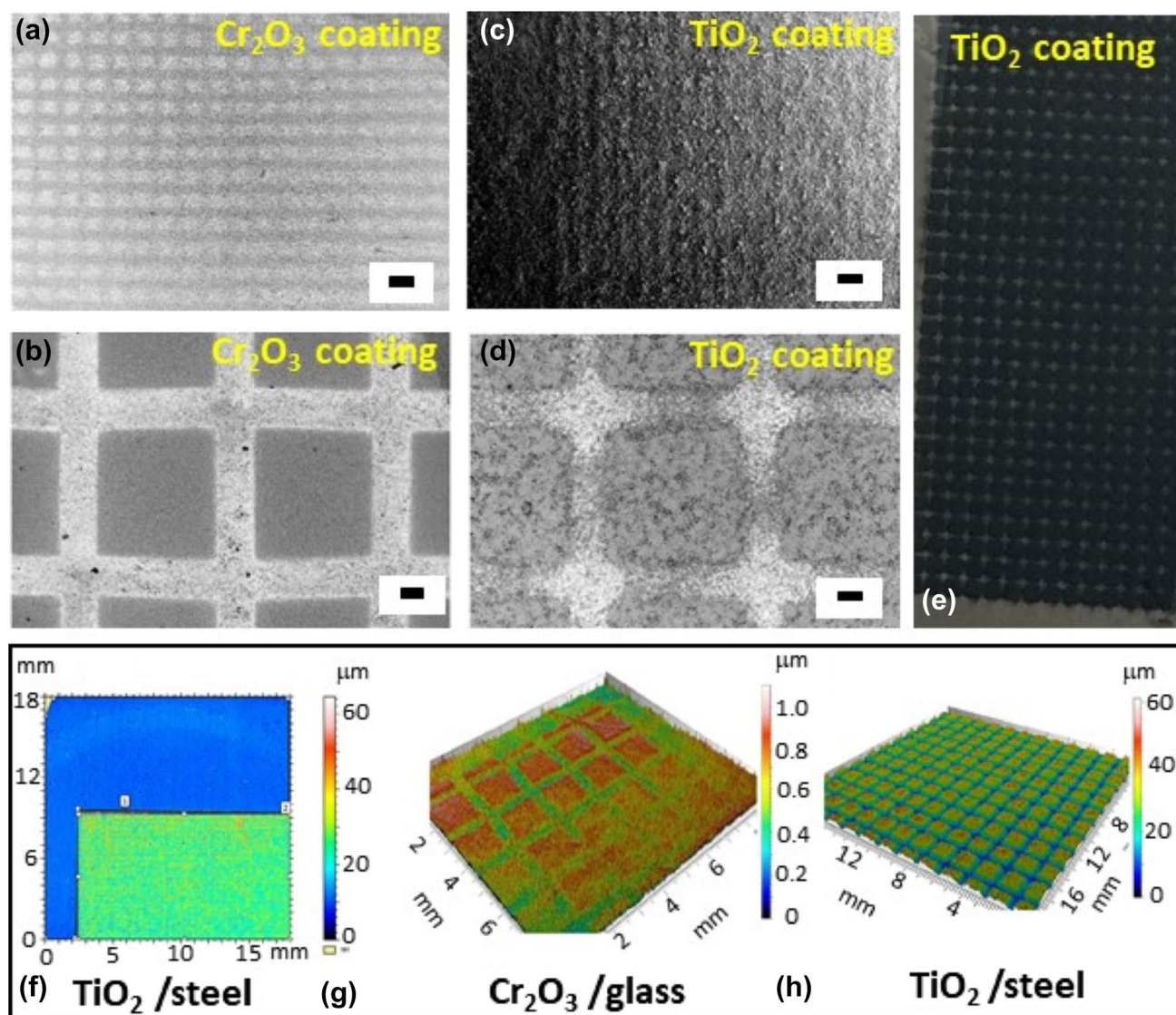
Fig. 2 Three-dimensional (3D) artificial periodic configuration; SEM micrograph of S-HVOF sprayed \text{Cr}_2\text{O}_3 coatings a aperture size 143 \mu\text{m} , b aperture size 1 mm; APS-sprayed \text{TiO}_2 coatings on mild steel substrate c aperture size 143 \mu\text{m} , d aperture size 1 mm; and e optical image of \text{TiO}_2 coatings. Scale bar equal to 200 \mu\text{m} ; non-
