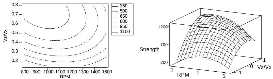
Graphical study of the response strength as a function of defined input variables of rotational speed and velocity ratio.
