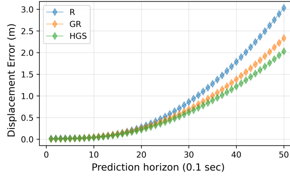
Figure 3: Results of the ablation study. State inputs: (x, y, v_x, v_y, \psi) . T_h = 30 (3 sec). T_f = 50 (5 sec).
