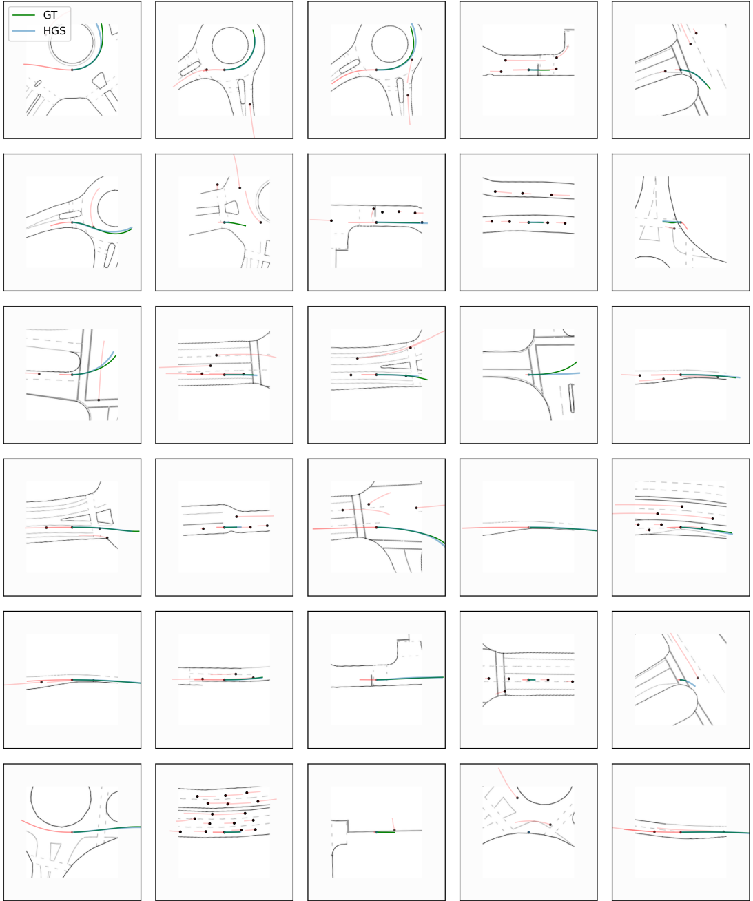
Figure 9: Visualized results of HGS using the INTERACTION validation dataset. Traceback horizon: T_h = 30 . Prediction horizon: T_f = 50 . Input data: (x, y, v_x, v_y) . Graphic encoder: GAT. Dynamics encoder: GRU. GT: Ground truth trajectory. HGS: HGS predicted trajectory. Black dots and red lines are current positions and historical tracks of vehicles.
