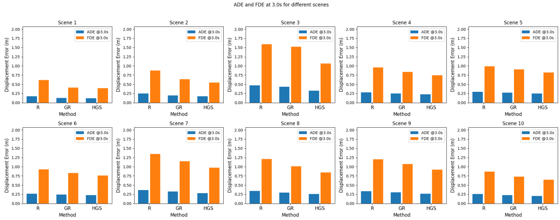
Figure 7: Results at 3 second. T_f = 30 (3 sec). Same setting as Fig. 6 except the prediction horizon.
