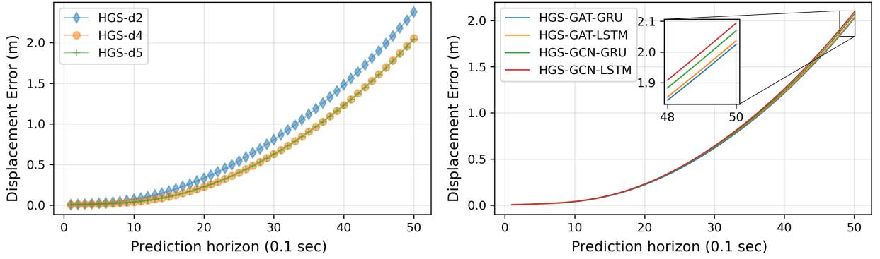
Figure 4: Left, Extendability of HGS. HGS-d2: HGS using (x, y) as input states; HGS-d4: HGS using (x, y, v_x, v_y) for input states; HGS-d5: HGS using (x, y, v_x, v_y, \psi) for input states. Right, Renewability of HGS. State inputs: (x, y, v_x, v_y) . T_h = 30 (3 sec). T_f = 50 (5 sec).
