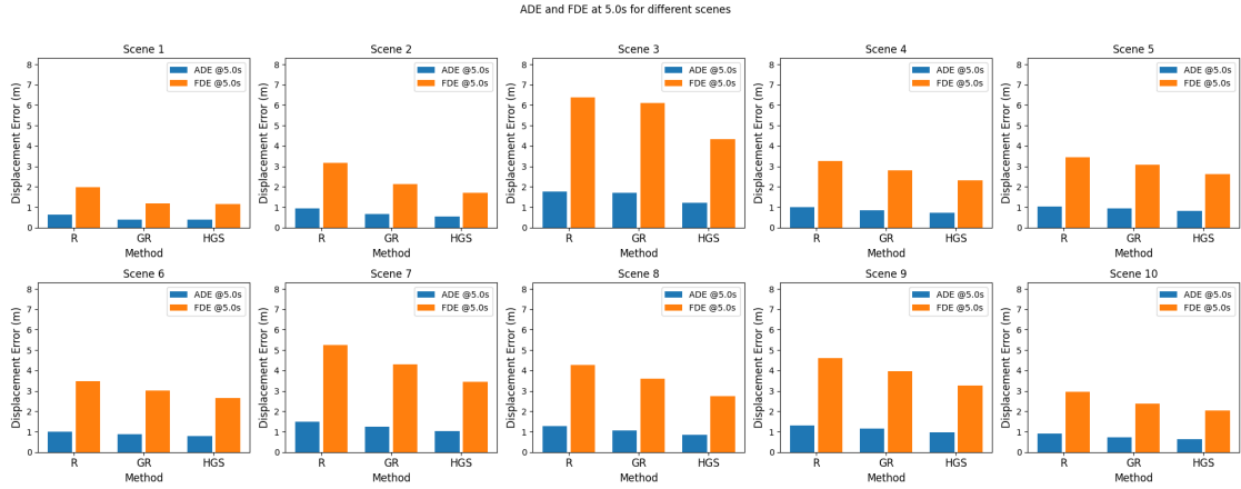
Figure 8: Results at 5 second. Prediction horizon: T_f = 50 (5 sec). Same setting as Fig. 6 and Fig. 7 except the prediction horizon.
