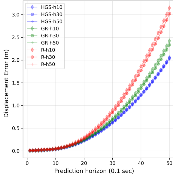
Figure 5: Impacts of traceback horizon. T_h = 10, 30, 50 (1, 3, 5 sec). T_f = 50 (5 sec). State inputs: (x, y, v_x, v_y) . HGS-GAT-GRU.
