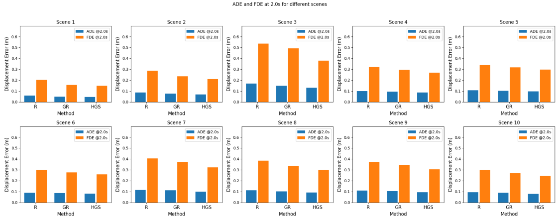
Figure 6: Results at 2 second. Traceback horizon: T_h = 30 (3 sec). T_f = 20 (2 sec). Same setting with Fig. 5 except the traceback and prediction horizons.
