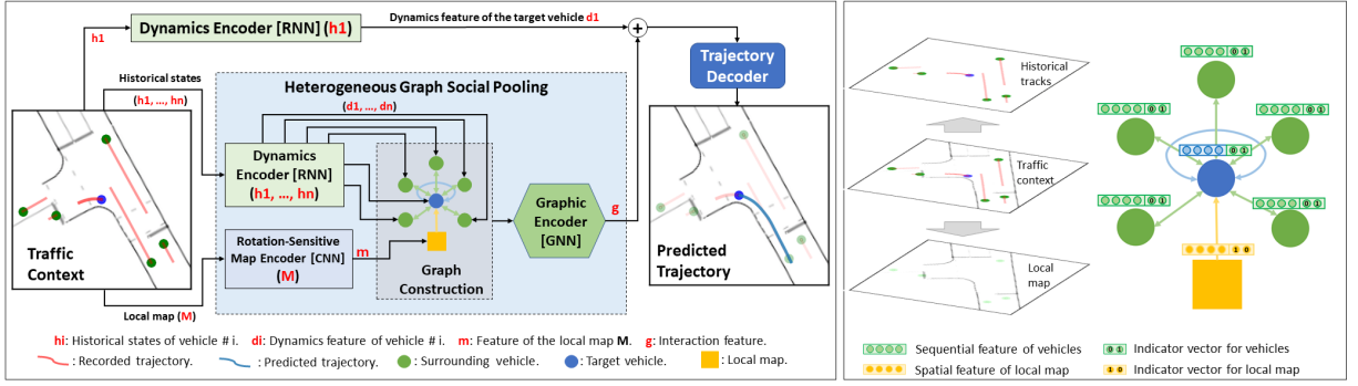
Figure 1: The proposed scheme with the constructed graph. Left , it consists of three encoders: a dynamics encoder (implemented using a recurrent neural network (RNN)) for vehicle dynamics feature extraction, a map encoder (implemented using a CNN) for understanding road structure information ( m ), and an HGS pooling (implemented using a GNN) for obtaining interaction features among traffic participants and the local map. The encoded dynamics ( d_1, \dots, d_n ) and interaction ( g ) features are then concatenated and sent to the trajectory decoder for trajectory prediction. Right , the traffic context is split into two parts: vehicles' historical states and the local map, and the target-centered heterogeneous graph is constructed with local connections.
