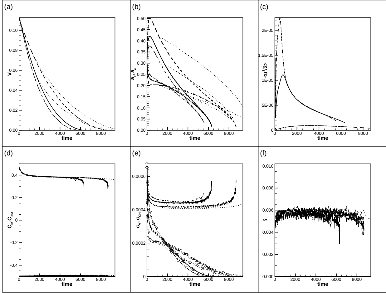
Figure 3: The droplet evolution at different Reynolds numbers. The results are shown for A = -0.5 , H = 3 , r_0 = 0.3 , Gr = 0.1 , Ca = 2.5 \cdot 10^{-5} , Pe = 5 \cdot 10^5 , and Re = 100 (dashed line), Re = 1000 (solid line), and Re = 2000 (dash-dot line). The dotted lines are obtained for the runs with neglected convective flows. The order of the graphs is as in figure 2.
