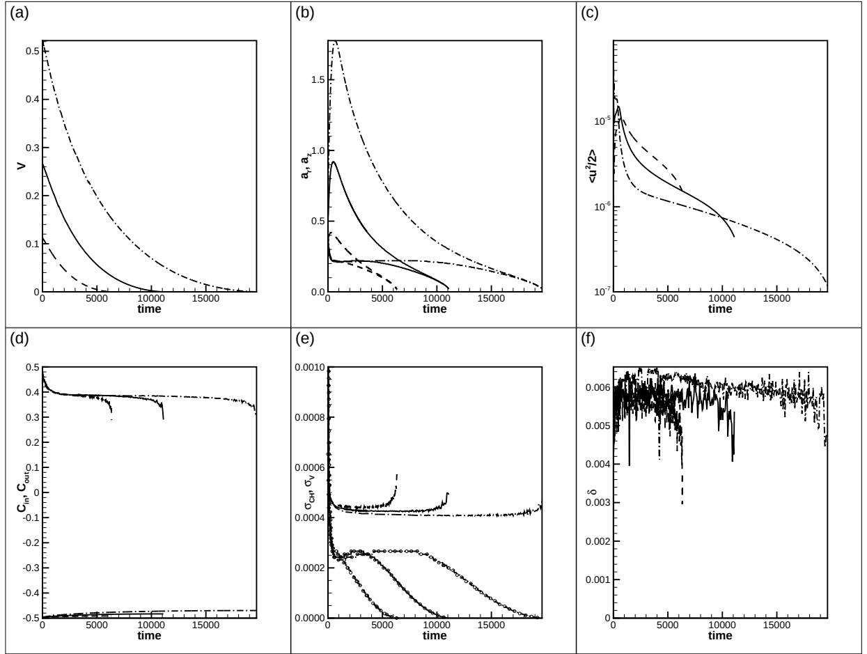
Figure 5: Time evolutions of the droplets of different sizes. The results are shown for A = -0.5 , H = 3 , Ca = 2.5 \cdot 10^{-5} , Pe = 10^5 , Re = 1000 , Gr = 0.1 , and r_0 = 0.3 (solid line), r_0 = 0.4 (dashed line), and r_0 = 0.5 (dash-dot line). The order of the graphs is as in figure 2.
