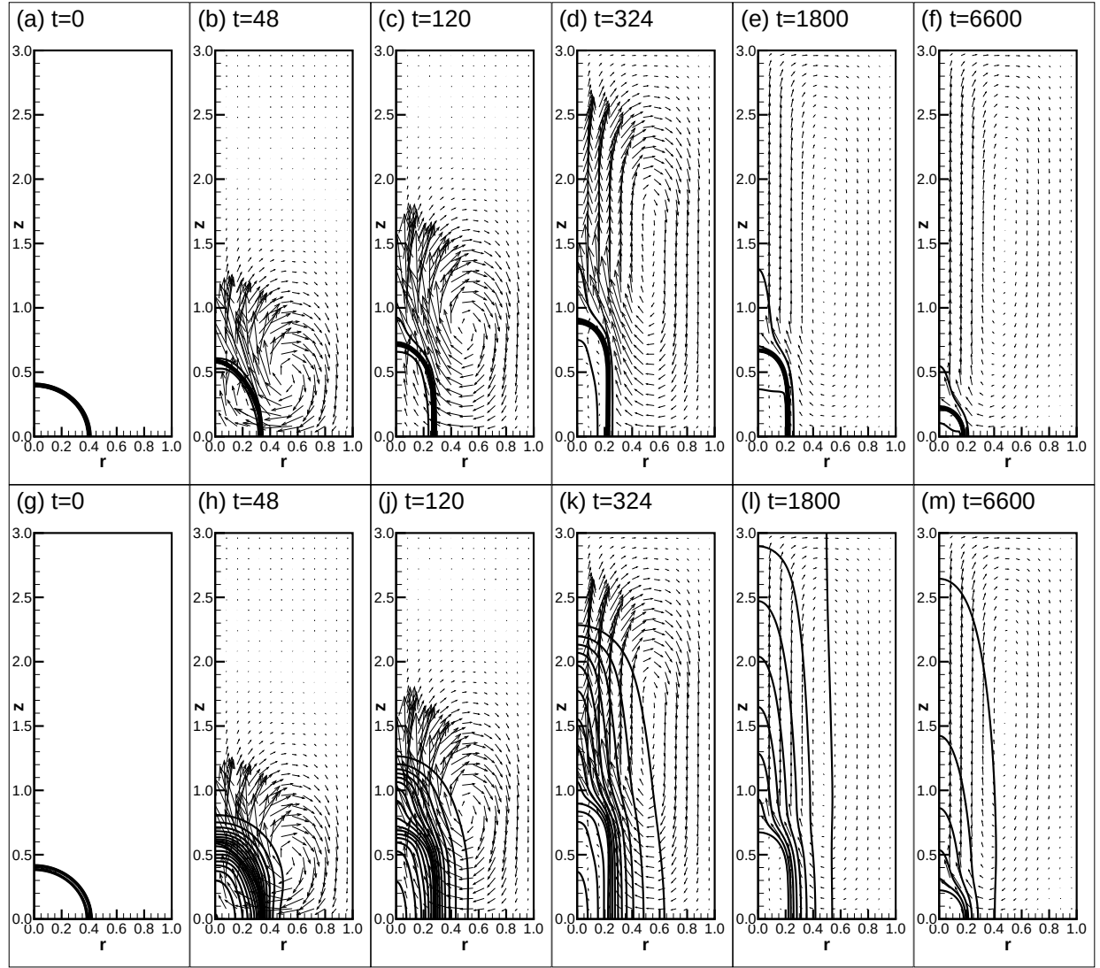
Figure 1: The snapshots of the fields of concentration, velocity, and chemical potential. The results are obtained for Re = 10^3 , Pe = 5 \cdot 10^5 , Ca = 2.5 \cdot 10^{-5} , A = -0.5 , H = 3 , Gr = 0.1 and r_0 = 0.4 . The upper row shows the fields of concentration and velocity and the lower row shows the fields of chemical potential and velocity. The time moments are indicated in the figure.
