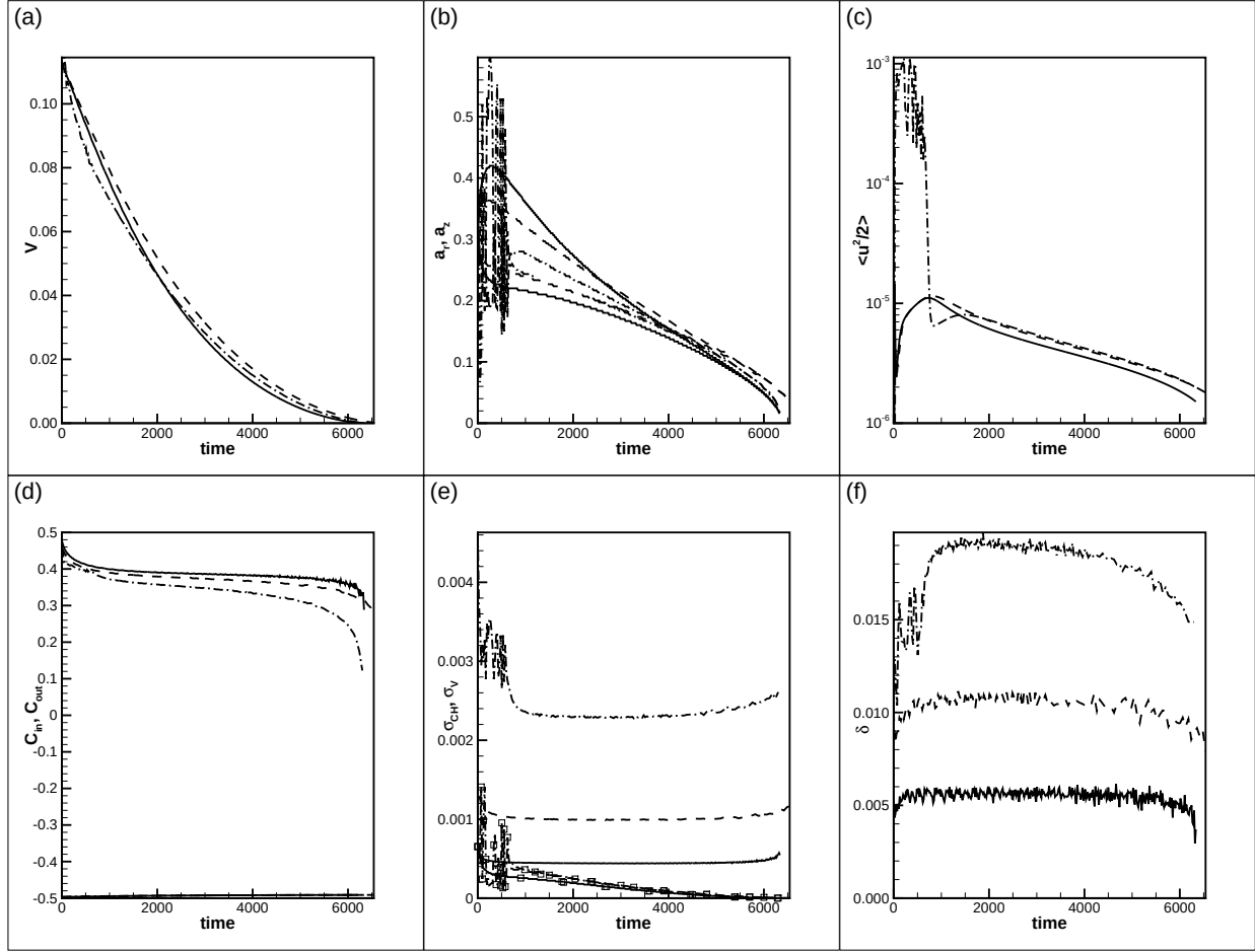
Figure 6: The droplet's evolution calculated for different capillary numbers. The results are shown for A = -0.5 , H = 3 , r_0 = 0.3 , Pe = 5 \cdot 10^5 , Re = 1000 , Gr = 0.1 , and Ca = 2.5 \cdot 10^{-5} (solid line), Ca = 10^{-4} (dashed line), and Ca = 4 \cdot 10^{-4} (dash-dot line). The order of the graphs is as in figure 2.
