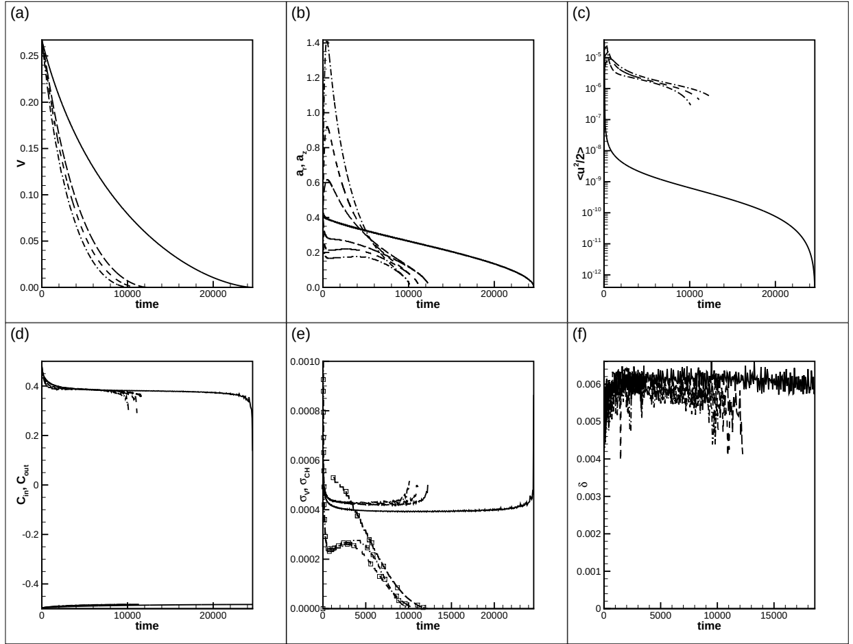
Figure 4: The droplet evolution at different Grashof numbers. The results are shown for A = -0.5 , H = 3 , r_0 = 0.4 , Ca = 2.5 \cdot 10^{-5} , Pe = 5 \cdot 10^5 , Re = 1000 , and Gr = 0 (solid line), Gr = 0.1 (dashed line), and Gr = 0.2 (dash-dot line). The order of the graphs is as in figure 2.
