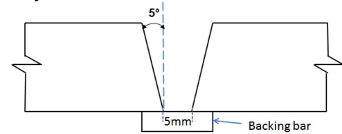
Figure 1. Welding setup preparation with backing bar
