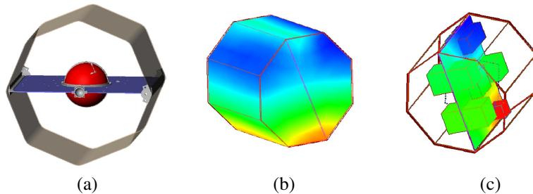
Figure 4 – (a) Main structural design and (b) & (c) thermal analysis.
