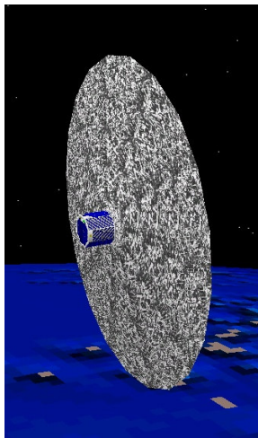
Figure 7 – The MUSTANG-2 spacecraft with the de-orbit device deployed.
