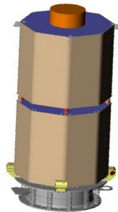
Figure 2 – The launch configuration of the two MUSTANG-2 spacecraft including the launch adapter.
