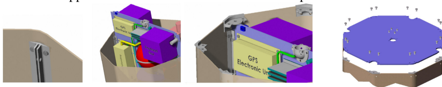
Figure 6 – Integration of the MUSTANG-2 spacecraft.
