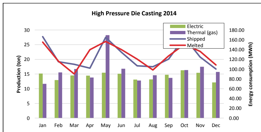
Figure 3: Example of energy data information captured by a high pressure die casting foundry in the UK
