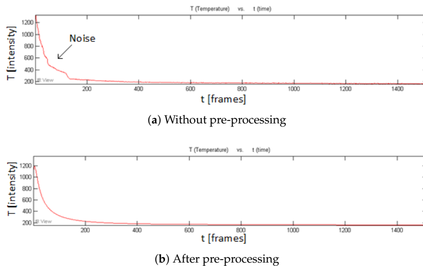
Figure 12. Temperature profile curves (cooling phase) in PT for CFRP 02.
