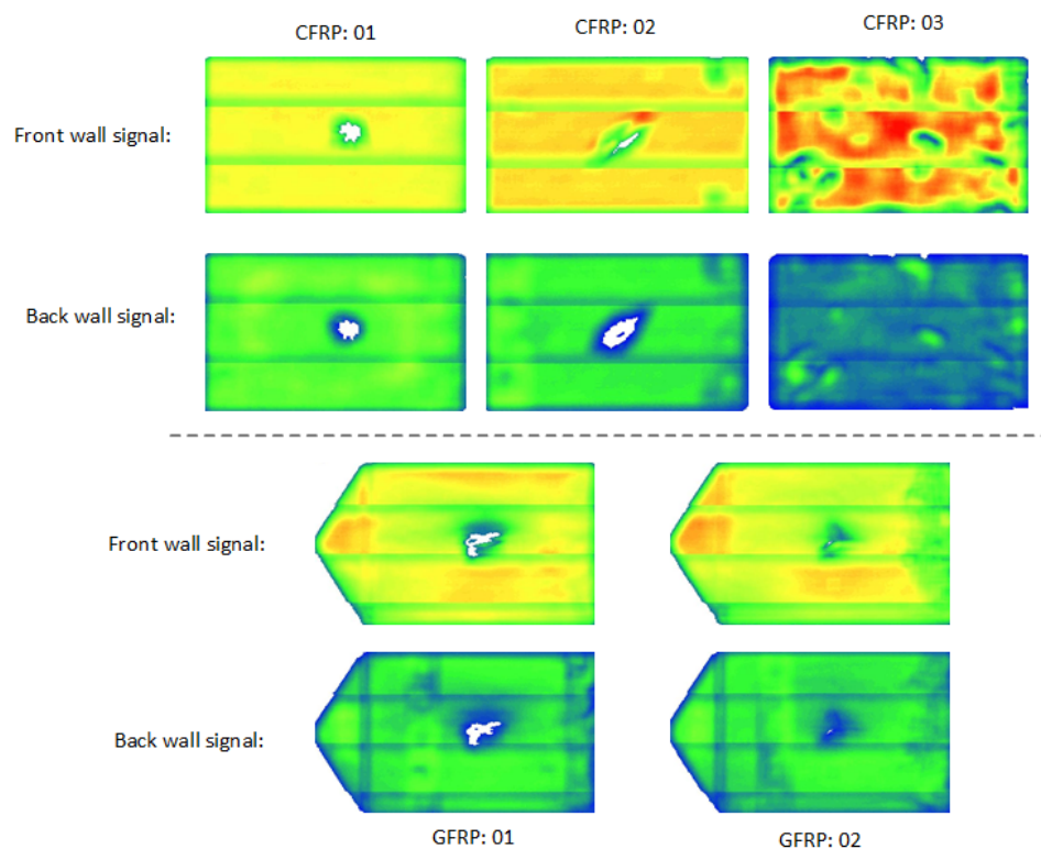
Figure 2. UT results.
