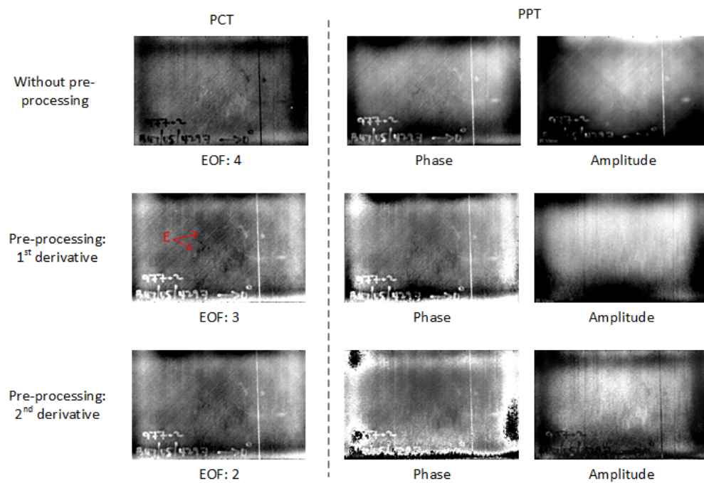
Figure 13. Thermographic results in PT for CFRP 03.
