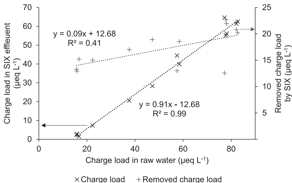
Fig. 6. Relationship between the charge load in the raw water and in the SIX treated water, along with the charge load removed.
