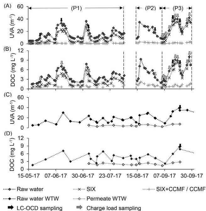
Fig. 1. Time series data for DOC and UVA removal for the pilot plant in (A) and (B) before treatment (raw water), after SIX treatment (SIX effluent) and after coagulation with membrane filtration (final water). Period (P1) operation with SIX and coagulation with membrane filtration (SIX + CCMF); P2 operation with CCMF only (no SIX pre-treatment); P3 operation with SIX + CCMF. UVA 254 (C) and DOC (D) of samples from Invercannie WTW before treatment and after coagulation and membrane filtration (permeate WTW).
