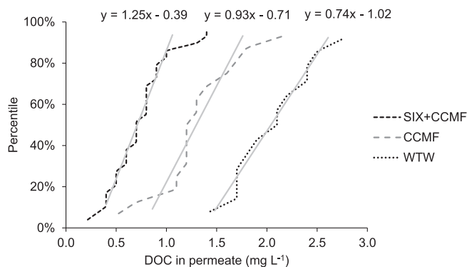
Fig. 2. Robustness of the different treatment methods shown as linear regressions (between 15 and 85%iles) in the cumulative frequency plot of the DOC in final water of SIX + CCMF, CCMF and permeate from the WTW.
