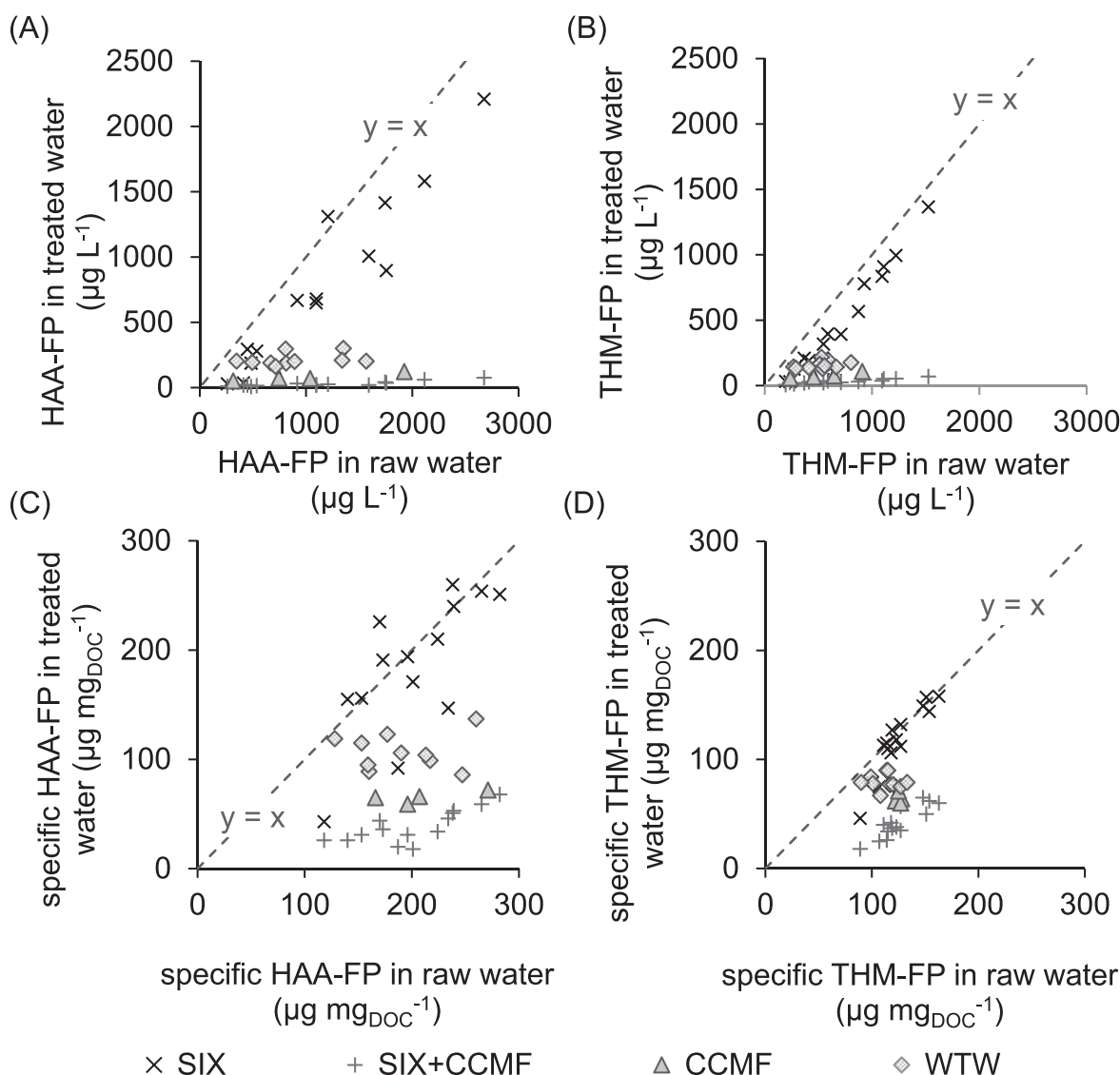
Fig. 3. DBP-FP of the water treated by different steps/methods as a function of their raw water DBP-FP for HAAs (A) and THMs (B), and DBP reactivity expressed as specific formation potential of the water treated by different steps/methods as a function of their raw water sDBP-FP for HAAs (C) and THMs (D).
