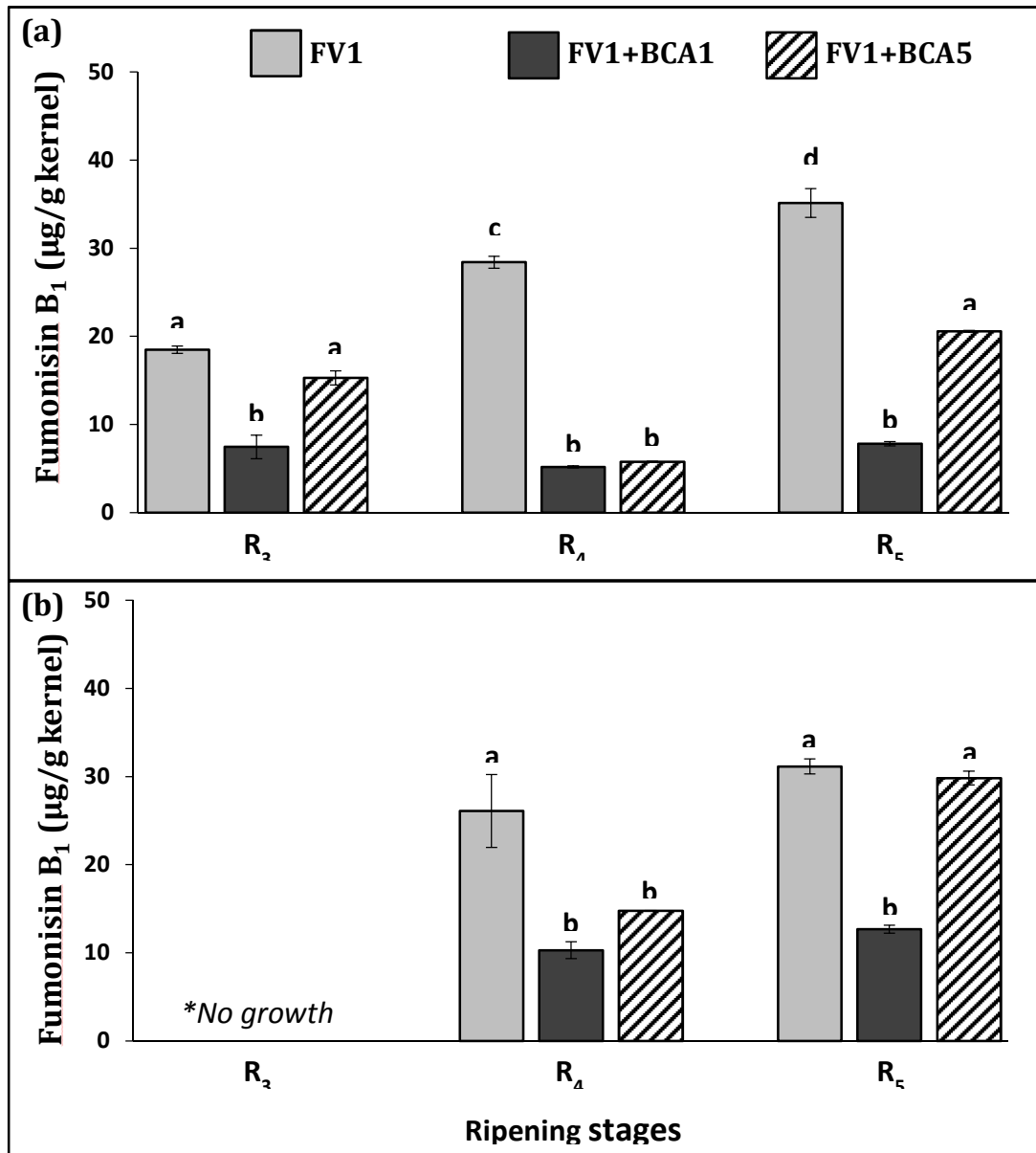
Figure 3. Fumonisin B 1 production by FV1, FV1+BCA1 (gram positive bacterium) and FV1+BCA5 ( C.rosea 016) on maize cobs of different ripening stages (R 3 , R 4 , R 5 ) after 10 days incubation at (a) 25°C and (b) 30°C. Data are means of triplicates. Bars are SEs. Different letters indicate significant difference (p ≤ 0.05) using Fisher's Least Significant Difference (LSD). Adapted from [9].
