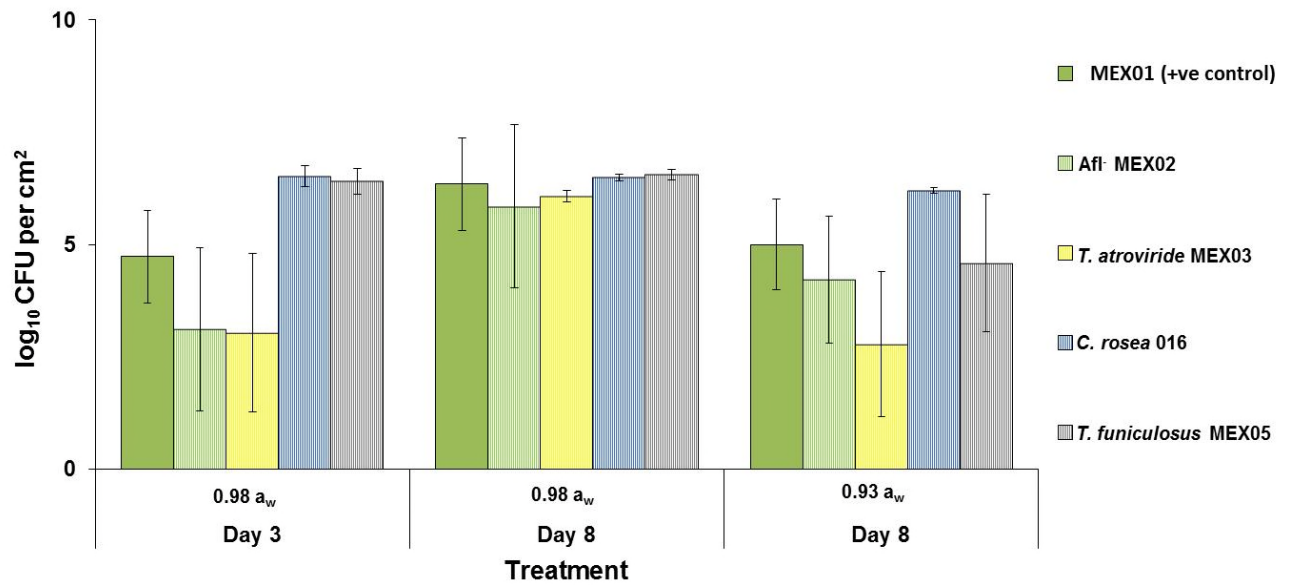
Figure 1. Sporulation of the toxigenic A. flavus strain (MEX01) ( \text{Log}_{10} conidia/ \text{cm}^2 ) during co-inoculation with different potential BCAs on senescent maize leaves at 0.98 (-2.8 MPa water potential) and 0.93 a w (-9.8 MPa water potential) at 30°C, harvested after 3 and 8 days. Bars indicate SEM. There were no significant difference ( p < 0.05 ) between treatments (Tukey's Honest Significant Difference).
