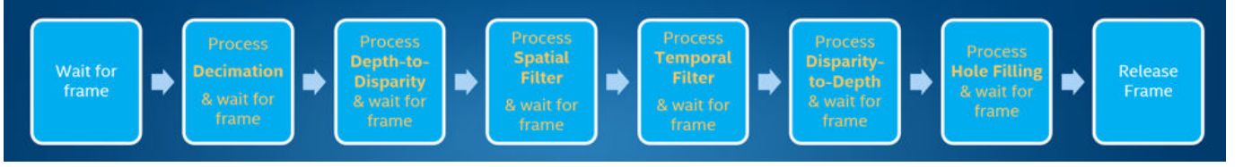
Fig. 10. Filter flowchart
