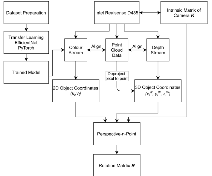
Fig. 2. PosEst workflow
