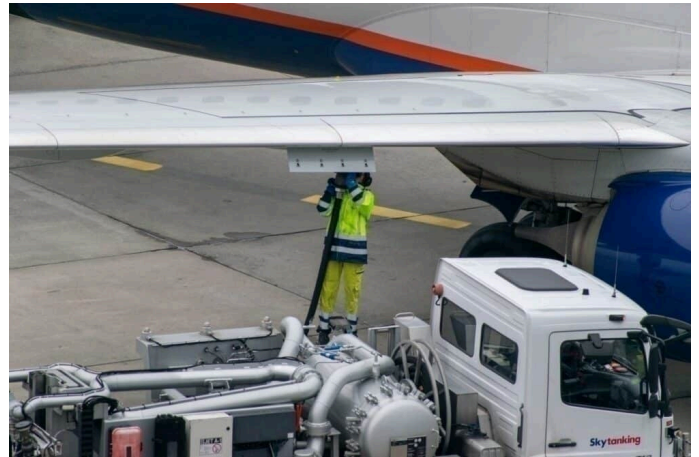
Fig. 1. Pressure aircraft refuelling
