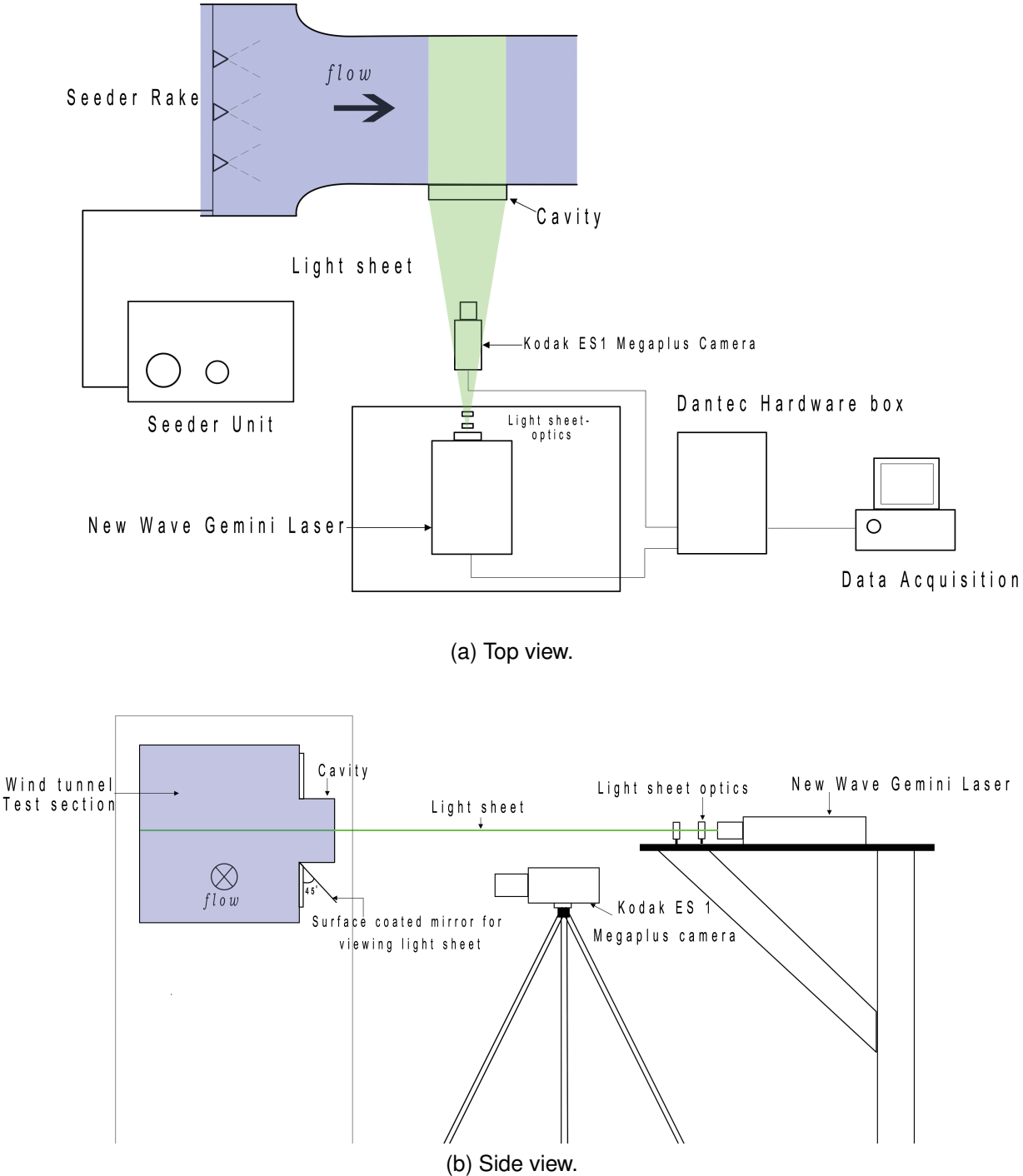
Figure 6: Schematic of the PIV setup.
