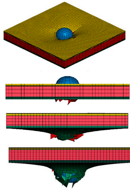
Fig. 11. Various stages of the impact of the striker on the sandwich panel with Design S1.
