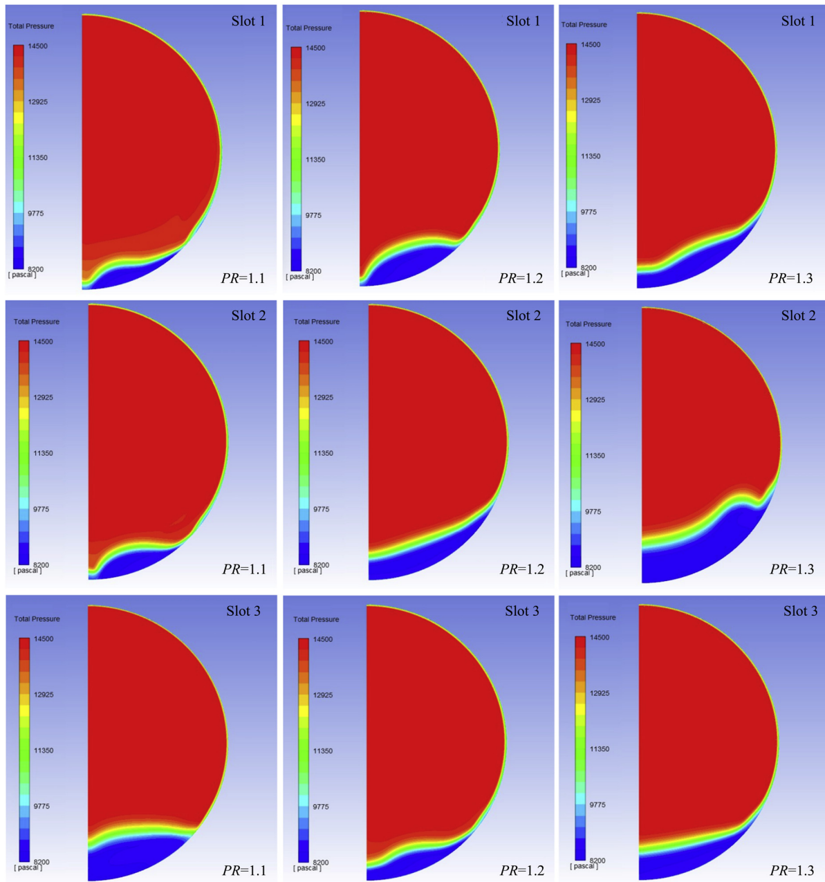
Figure 14 Effect of slot blowing on the fan_face total pressure (Pa) contours, using Slot 1, Slot 2 and Slot 3 with a strong intake separation at 20^\circ angle of attack, at different pressure ratios.
