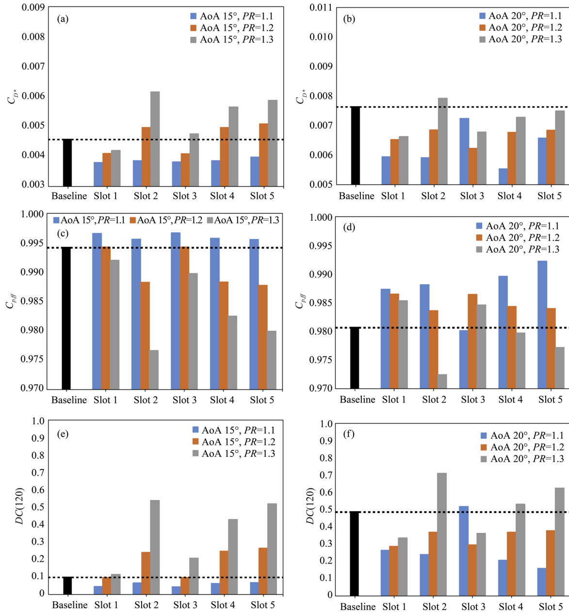
Figure 12 Effect of each slot variant on the modified drag coefficient ( C_{D^*} ), DC(120) distortion and total pressure coefficient ( C_{p,eff} ), at angle of attack 15° and 20° for different blowing pressure ratios.
