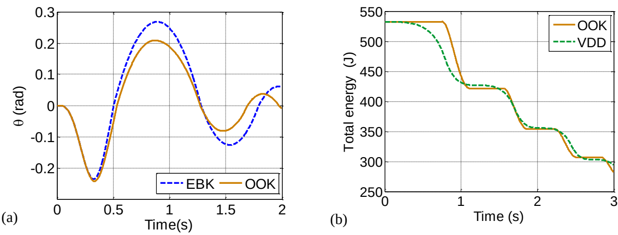
Fig.8. (a) Time-history of a rigid block (BLC05) anchored with constant (EBK) and on-off restraint systems (OOK); (b) time-history of the total energy of a rigid block (BLC05) with on-off restraint system (OOK) and with damper device (VDD).
