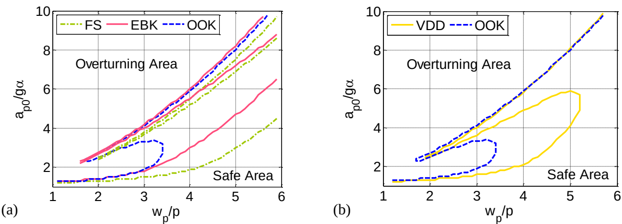
Fig.13. Overturning spectra of BLC06 evaluated for different restraint conditions: free-standing (FS); anchorages with elastic-brittle stiffness (EBK); anchorages with on-off stiffness (OOK); viscous damper devices (VDD).
