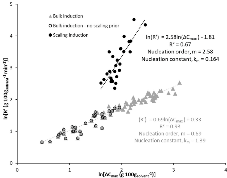
Fig. 10. Establishing the relationship between metastable zone width (MSZW, \Delta C_{\max} ) and supersaturation rate ( R' ) at induction based on interfacial concentrations for: (i) bulk induction (distinguished between data where scaling was also present or absent); and (ii) scaling induction (black closed circles). Complete dataset ( T 45–60 °C, \Delta T 15–30 °C) is shown for bulk nucleation which occurred irrespective of scaling.
