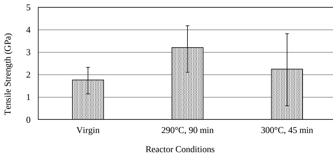
Figure 4. Single fibre tensile tests of carbon fibres recovered after processing at 290°C, 90 min and 300°C, 45 min
