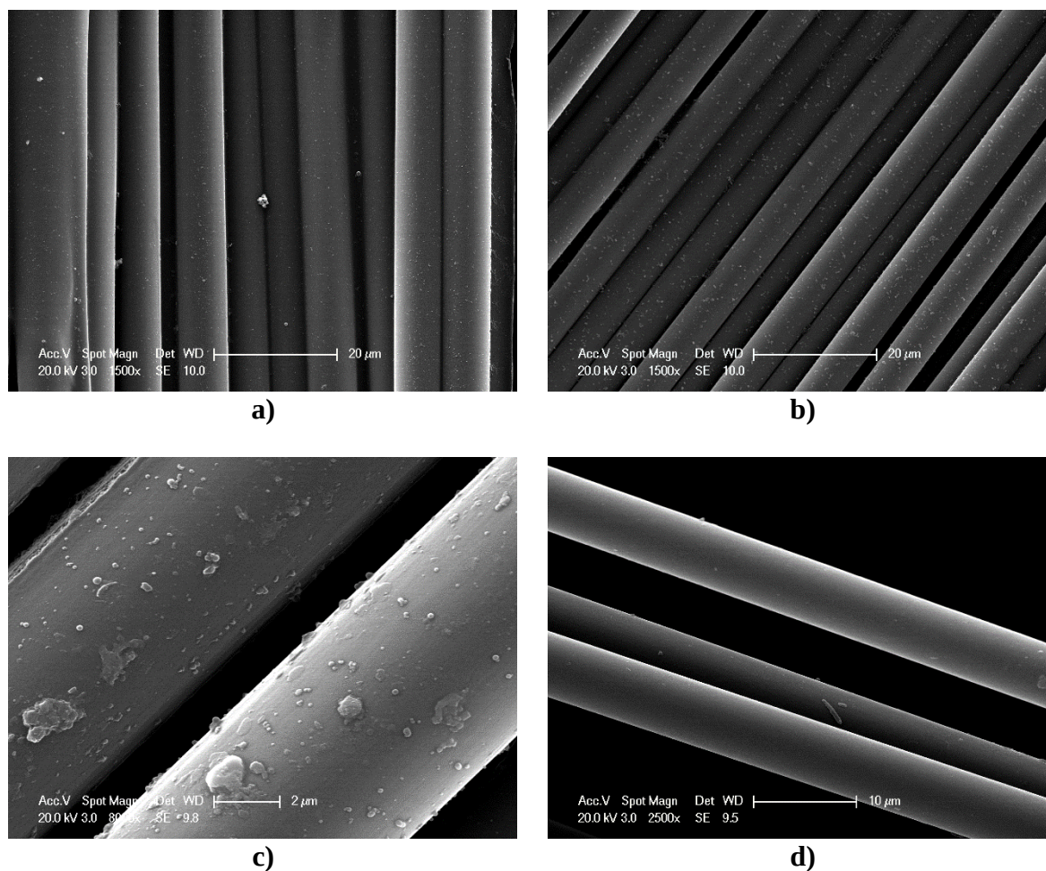
Figure 3. SEM images of fibres recovered after processing with an acetone/water solvent and \text{ZnCl}_2 catalyst at a concentration of a) 0.05 M; b) and c) 0.10 M and d) 0.10 M with light wash with water.
