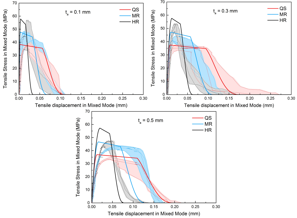
Figure 19: Validation of the model (solid line) against the experimental results (shaded area) for a thickness of: (a) t_a = 0.1 mm, (b) t_a = 0.3 mm and (c) t_a = 0.5 mm in mixed-mode.
