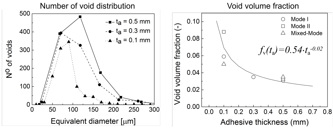
Figure 6: Results of computer tomography X-ray scans for representing the void distribution of the investigated bondline thicknesses t_a = 0.1, 0.3 and 0.5 \text{ mm} , the number of voids over the equivalent void diameter and the void volume fraction.
