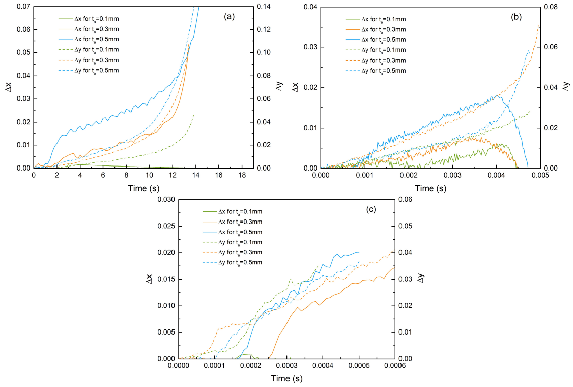
Figure 18: Experimentally obtained relative displacements for a) quasi-static, b) medium-rate and c) high-rate loading regimes for three investigated adhesive thicknesses.
