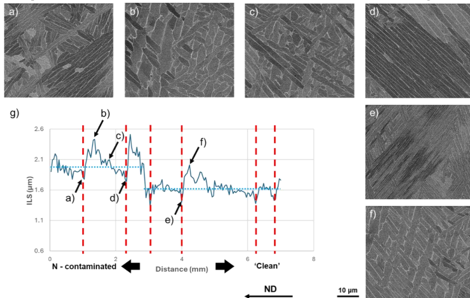
Figure 2. (a-d) Sequential SEM-BSE images showing the microstructure from one HAZ band to another. (e) and (f) are two SEM-BSE images showing the microstructure across one HAZ band from the clean section. (g) Linear intercept \alpha -lamellar spacing (ILS) measurement across 6 HAZ bands across the interface taken from the position highlighted in figure 1(b) by the white arrow.
