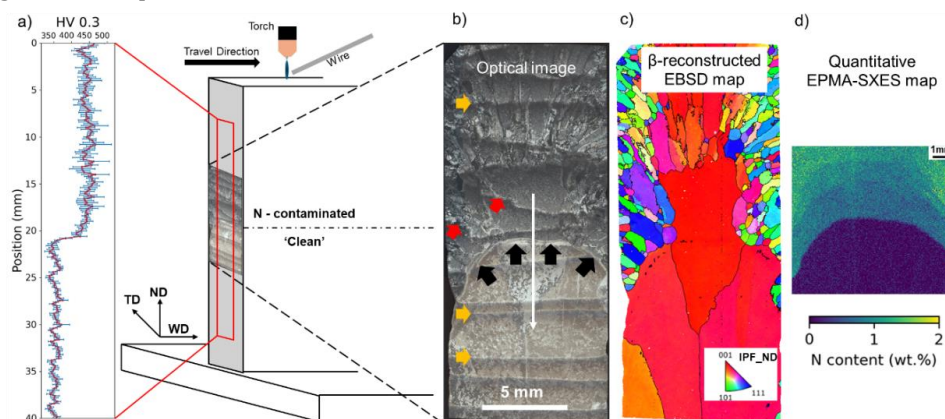
Figure 1. (a) N-contamination WAAM wall schematic diagram and reference frame, alongside a hardness profile on the ND across the interface. (b) An optical image taken from the interface. Fusion boundary between clean and contaminated part is indicated by black arrows. Some HAZ bands are highlighted by red and orange arrows. (c) A \beta -reconstructed EBSD map of the same area. (d) Quantified EPMA-SXES map showing N level at the interface. The white line on the optical image indicates where the SEM-BSE scanning was performed (figure 2).
