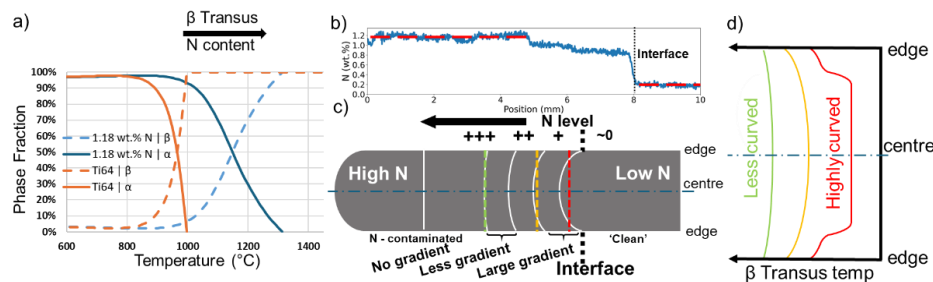
Figure 3. (a) A diagram showing the \beta -transus temperature of Ti64 (no contaminants) and Ti64 with higher N content (1.18 wt.% as given by EPMA). (b) A line profile of a longer higher spatial resolution EPMA map to show the N content on each part and the gradient along ND. (c) A schematic illustration of the distribution of the N gradients along the ND and (d) a schematic diagram showing T_{\beta} profiles relating to HAZ band behaviour.
