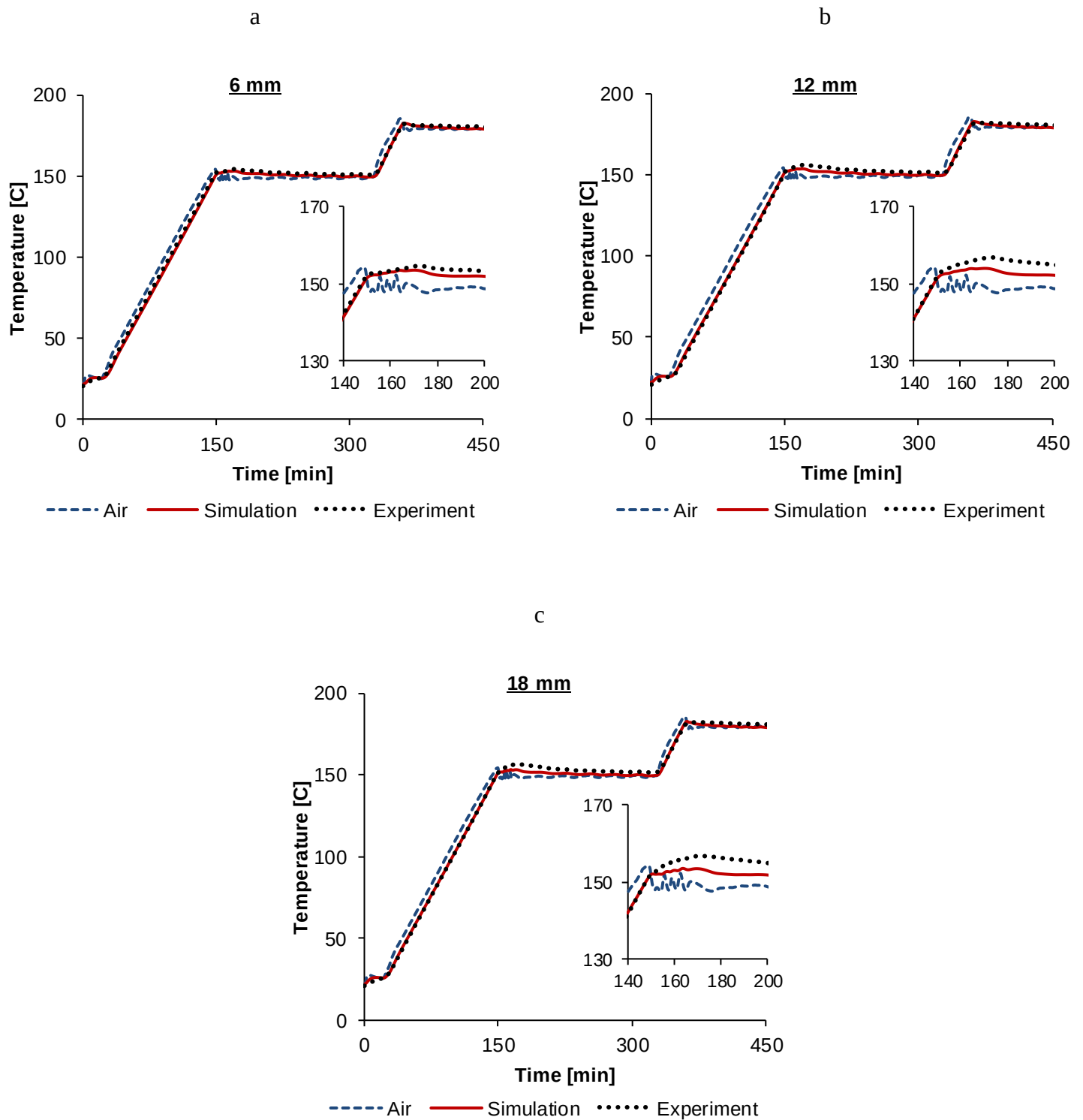
Figure 9. Cure cycle 2: simulated and measured temperature evolution in the thick composite sample. Insert shows a small exotherm at the beginning of the 150°C dwell.
