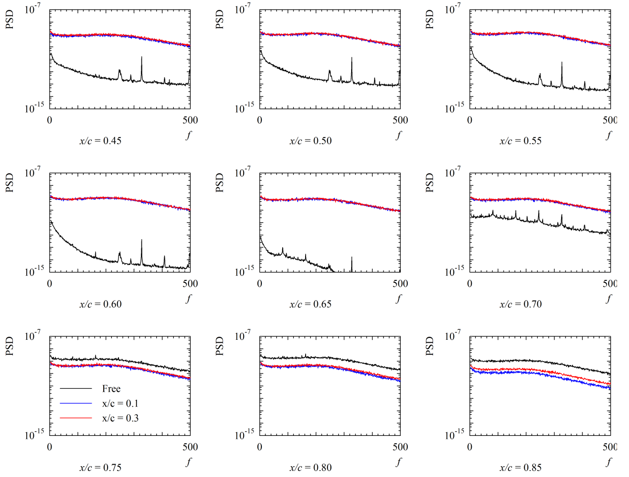
Fig. 6 PSD of quasi-wall-shear stress for free- and forced-transition cases at \alpha = 0^\circ ( Re_c = 6 \times 10^5 )
