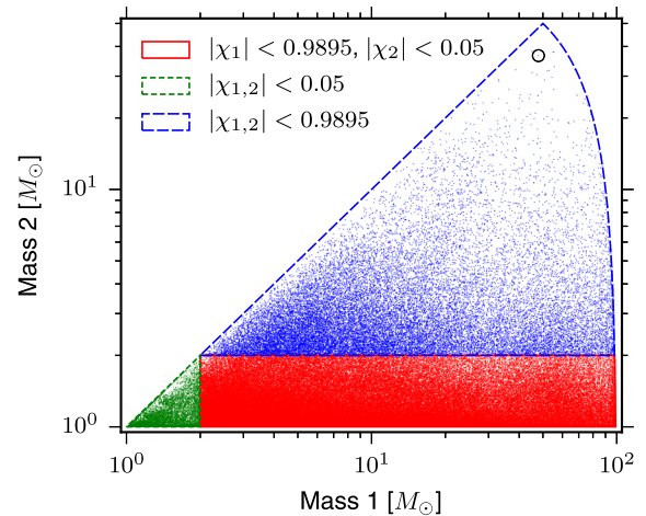
FIG. 1. The four-dimensional search parameter space covered by the template bank shown projected into the component-mass plane, using the convention m_1 > m_2 . The lines bound mass regions with different limits on the dimensionless aligned-spin parameters \chi_1 and \chi_2 . Each point indicates the position of a template in the bank. The circle highlights the template that best matches GW150914. This does not coincide with the best-fit parameters due to the discrete nature of the template bank.
