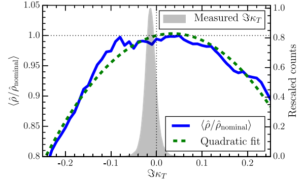
FIG. 9. Variation in \hat{\rho} when the time-dependent parameter \Im \kappa_T is adjusted. The solid blue curve represents \hat{\rho} averaged over 16 software injections, with waveform parameters identical to the best-fit template for GW150914. \hat{\rho} decreases as \Im \kappa_T deviates from its nominal value. The green dashed curve is a quadratic fit, and represents the approximate behavior of \langle \hat{\rho} \rangle if we had used a much larger number of software injections. The gray histogram represents the measured values of \Im \kappa_T for times used in the analysis on September 14 and 15.
