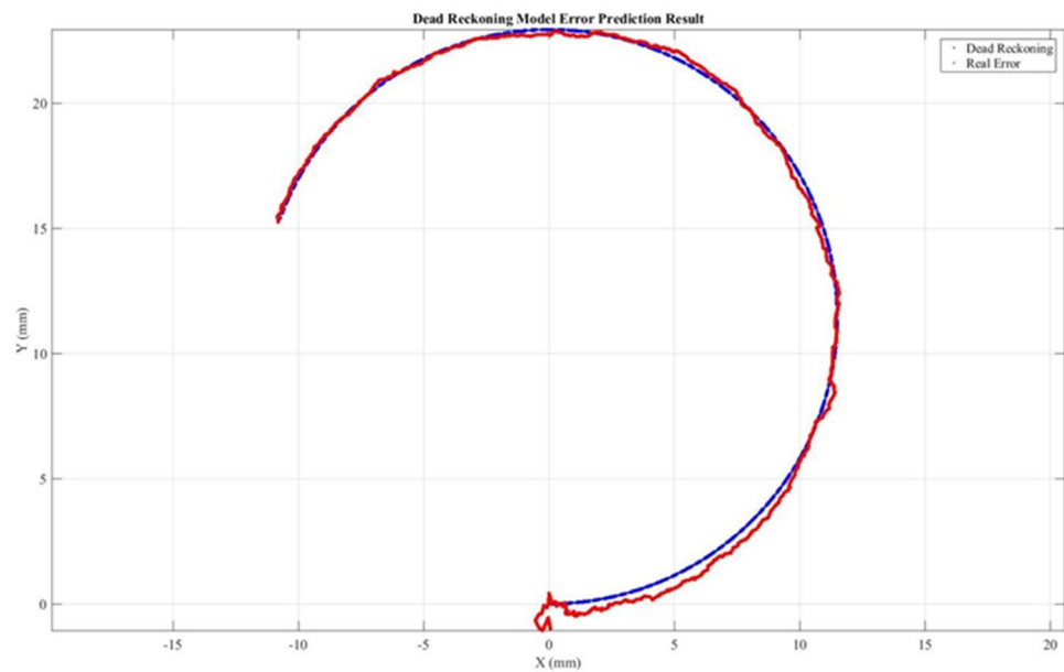
Figure 9. Dead Reckoning Model Error Prediction Result.
