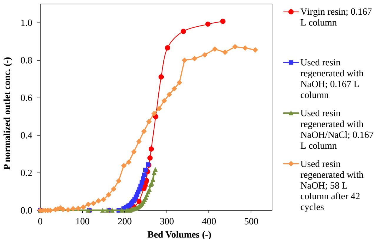
Fig. 2 - Breakthrough curves obtained in the lab-scale (0.17 L) and demonstration scale (58 L) columns, shown as outlet P normalized concentration versus the BVs fed to the column. Initial P concentrations were: 7.1 \pm 0.2 \text{ mg}_P \text{ L}^{-1} for virgin resin, 6.6 \pm 0.2 \text{ mg}_P \text{ L}^{-1} for the used resin regenerated with NaOH and 6.9 \pm 0.1 \text{ mg}_P \text{ L}^{-1} for used resin regenerated with NaOH/NaCl.
