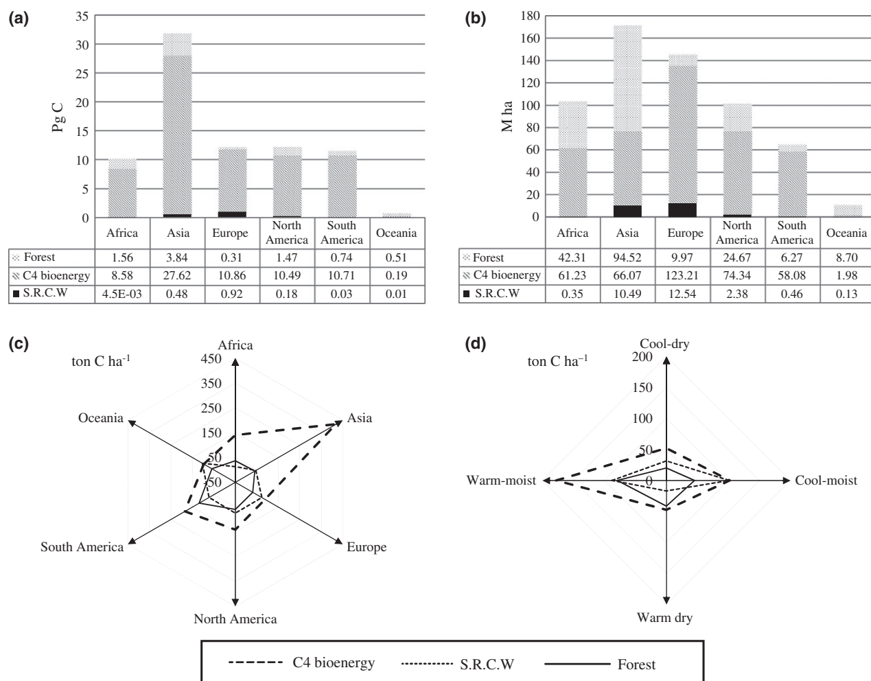
Fig. 2 Potential climate change mitigation of forest, C 4 bioenergy crop and short rotation coppice wood partitioned across global continental regions. In (a), the cumulative climate mitigation potential of forest includes biomass and soil C sequestration (Pg C) over 20 years, while the climate mitigation potential of bioenergy crops includes the fossil fuel C equivalent displaced by the use of bioenergy crop biomass (Pg C eq oil) and the sequestration of C in soil. In (b), the total extent of agricultural land (Mha) depends upon the capacity of each ecosystem to provide the highest climate mitigation potential. In (c), the potential climate mitigation of each ecosystem is reported on a per hectare basis discriminated among continents (for forest t C ha -1 , for bioenergy crops t C eq oil ha -1 ). In (d), potential climate mitigation of each ecosystem is reported on a per hectare basis and discriminated among climatic regions. SOC changes in the LUC transition to bioenergy crops plantations were assumed to increase of 18% and to forests were assumed to increase by 53% (Guo & Gifford, 2002). Peak yields of C 4 bioenergy crops from LPJmL were adjusted using a correction factor of 0.66 to obtain harvestable yield.
