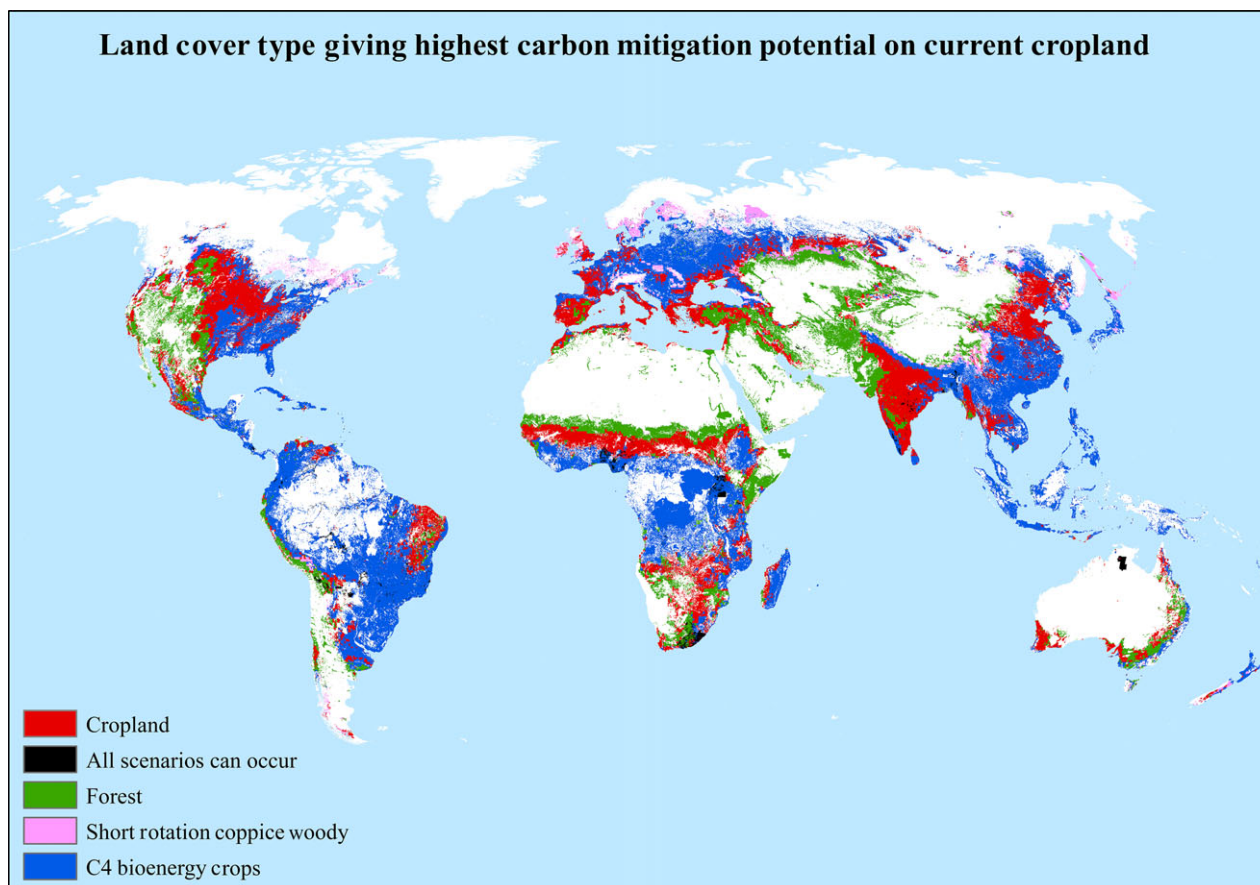
Fig. 3 Five-arc minute ( \approx 10 km at the equator) map of land-cover types giving the highest climate change mitigation potential C_4 bioenergy crops ( \approx 484.9 Mha), short rotation coppice wood ( \approx 26.3 Mha) and forest ( \approx 186.5 Mha). Red pixels indicate highly productive agricultural land not suitable to land-use change due to negative or neutral C stock difference when converted to C_4 bioenergy crops, short rotation coppice wood ( \approx 420.6 Mha). The pixels in black colour report agricultural land where both C_4 bioenergy crops and short rotation coppice wood have similar climate mitigation potential and could potential occur ( \approx 24 Mha).
