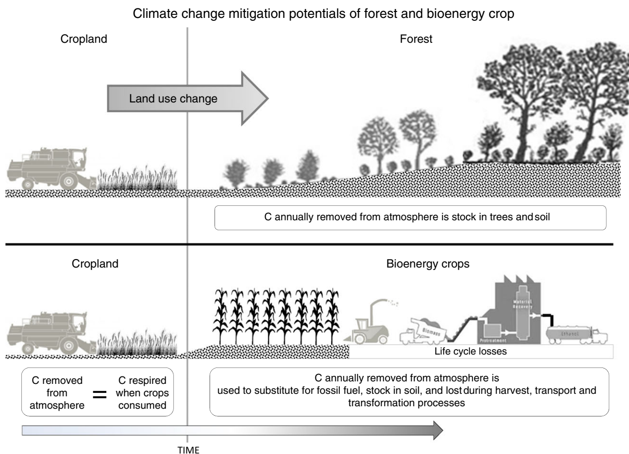
Fig. 1 Croplands do not accumulate carbon for more than a year, as their yields are in general respired within the same year of harvest. The climate change mitigation potential achievable in agricultural land strongly depends on the availability of land for food to be reforested or to be converted to bioenergy production. Forests have been reported to hold up to 50 times more C than a hectare of crop (Houghton, 2002) and depend upon the capacity of sequester C in biomass and soils relative to their agricultural productivity and the risks to be released back into the atmosphere through fire, harvesting and land clearance. The net climate mitigation potential of converting cropland to bioenergy crops is based on the ability of replacing fossil fuels for energy production through bioenergy production and the capacity to sequester additional C in agricultural soils during the 20 years of permanence in the ground. The displaced fossil fuel C equivalent ( C_{eq} oil) emissions are equal to the C emissions of the functionally equivalent fossil energy system minus the fossil C_{eq} emissions of the bioenergy system, for example due to harvest, transport and processing of the biomass.
