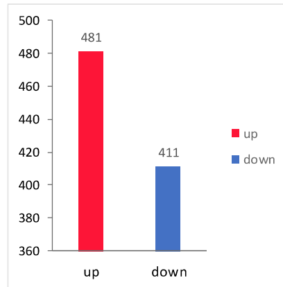
Figure 3: up and down differentially expressed genes (DEGs) between asparagus cv. Aspalim spears displaying tip breakdown and healthy spears, both grown at 14 °C night and 28 °C day and stored at 7 °C for 14 days (p adj <0.05).
