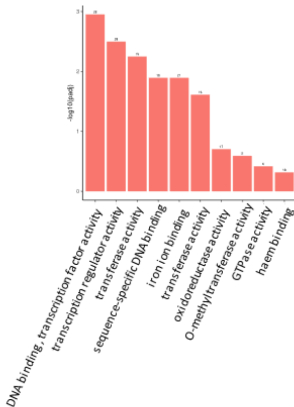
Figure 4: GO enrichment analysis of DEGs between asparagus cv. Aspalim spears displaying tip breakdown and healthy spears, both grown at 14 °C night and 28 °C day and stored at 7 °C for 14 days showing the GO category “molecular function”
